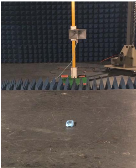
Radiated emissions test > 1GHz
