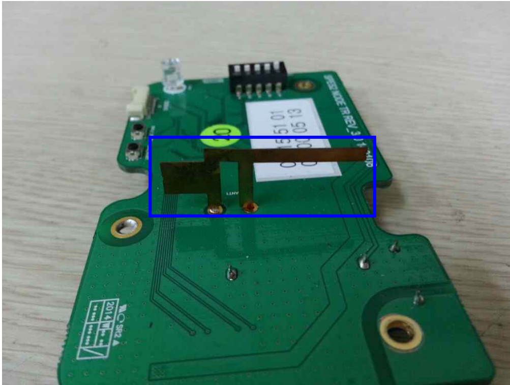
Zigbee Antenna
