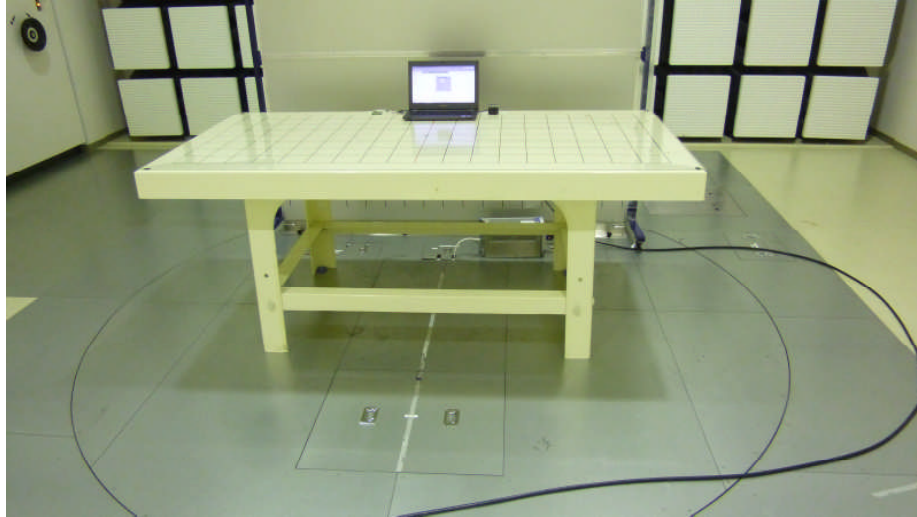
Photo3 Test Setup for Conducted Test_1 (Front)
