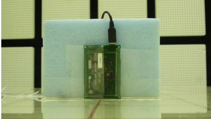
Photo1 Test setup for EUT
