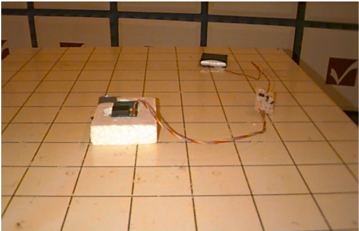
View of the T900 during the Radiated Emissions tests. PC board TX (green PCB) with dc supply / battery.
