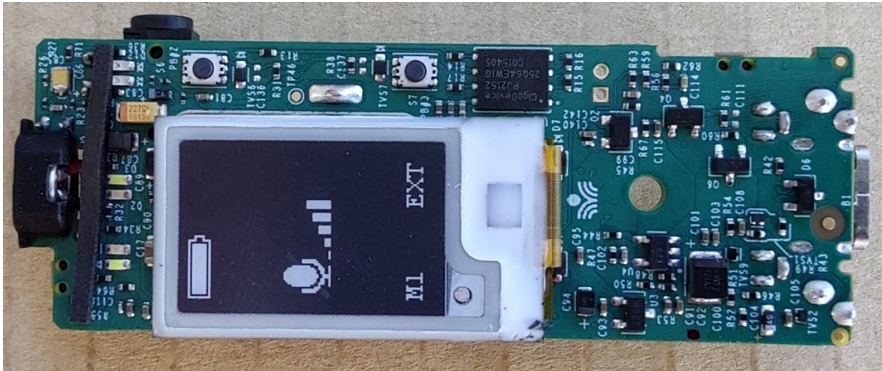
PCBA side 2 A
