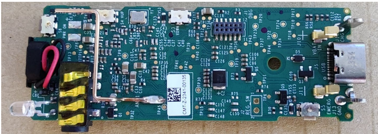
PCBA side 1
