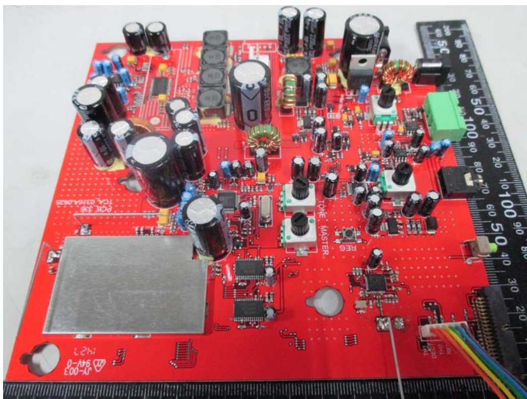
6. Front view of PCB
