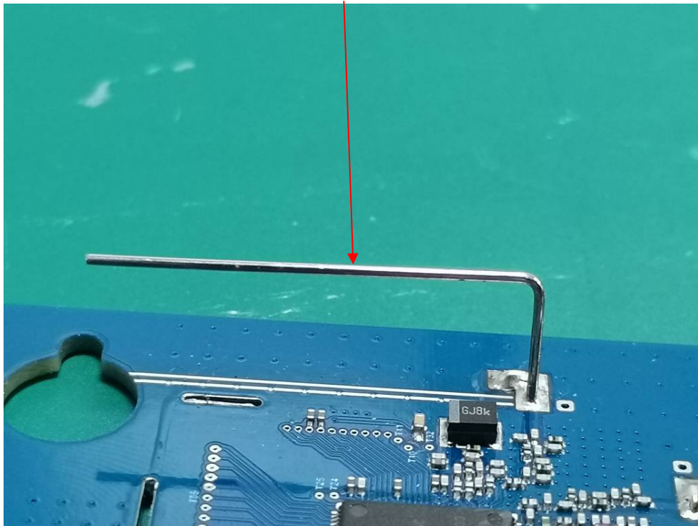
Antenna 1
