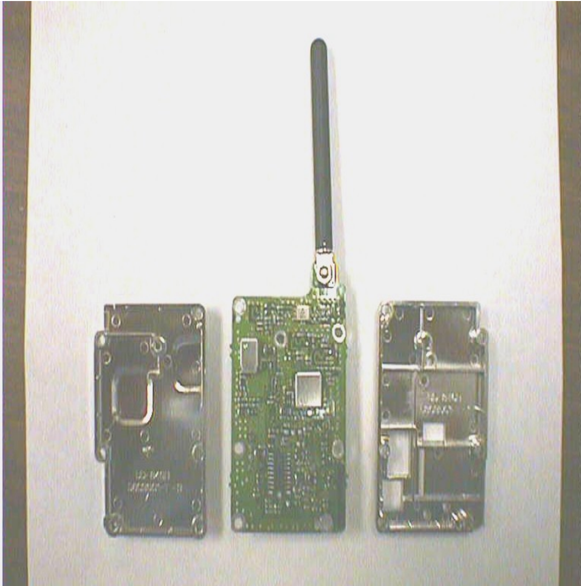
Ewave, Inc. Model: RF-10K Transceiver Internal product photo Top Level Assembly uncased
