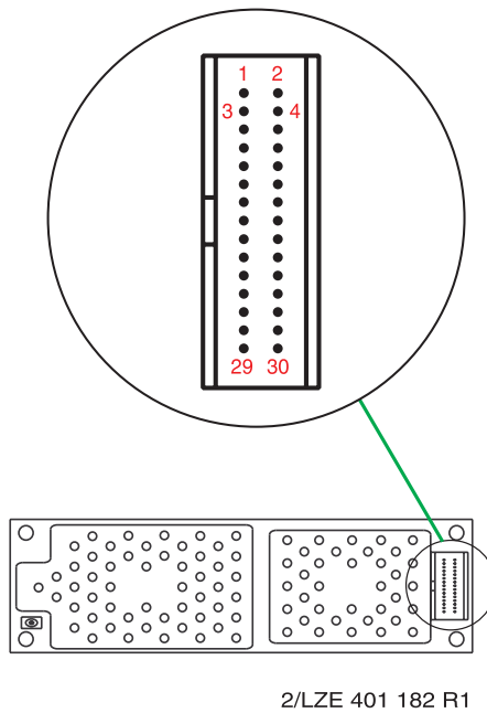
Figure 9 System connector - pin orientation
