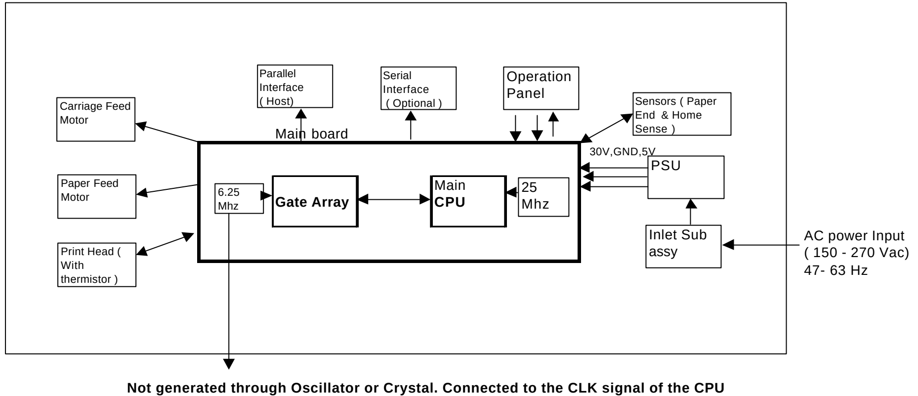
MSP 250 XLC PRINTER BLOCK DIAGRAM
