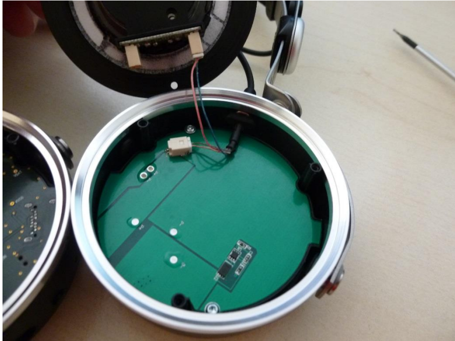
Photo 3: PCB 1 front side view
