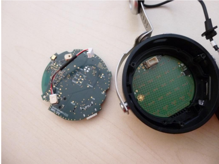
Photo 11: PCB 2 removed
