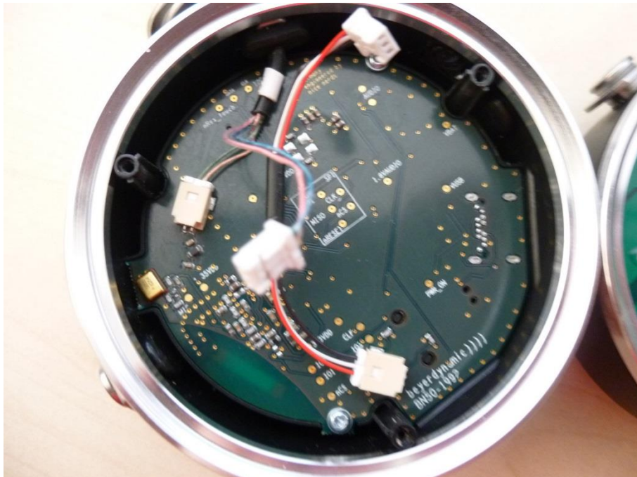
Photo 6: PCB 2 front side view
