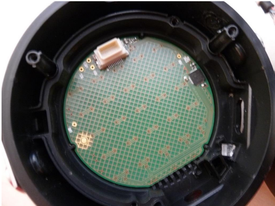
Photo 12: PCB 3
