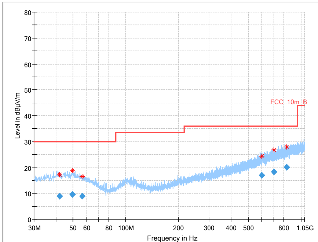
Plot 2: 30 MHz to 1 GHz, TX mode, 2480 MHz, vertical & horizontal polarization
