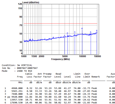
Headset 2.4G SRD_2M_TX_CH_39_Vertical-Peak
