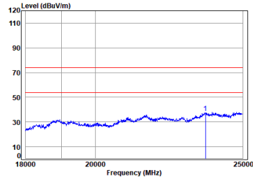
Headset 2.4G SRD_1M_TX_CH_19_Vertical-Peak
