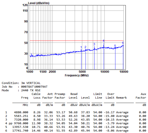
Headset 2.4G SRD_1M_TX_CH_19_Vertical-Avg
