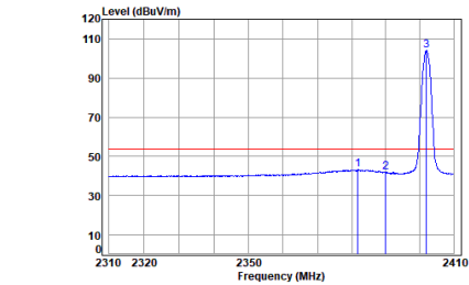
Headset 2.4G SRD_1M_TX_CH_00_Vertical-Avg
