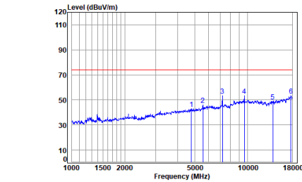
Headset 2.4G SRD_1M_TX_CH_00_Vertical-Peak
