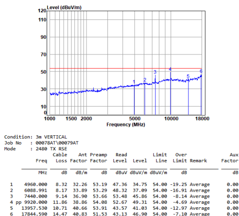
Headset 2.4G SRD_1M_TX_CH_39_Vertical-Avg
