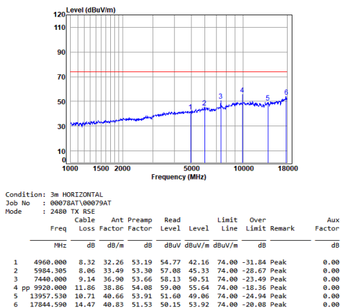
Headset 2.4G SRD_1M_TX_CH_39_Horizontal-Peak
