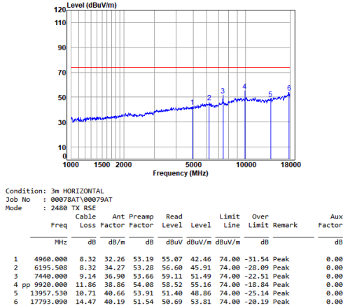
Headset 2.4G SRD_2M_TX_CH_39_Horizontal-Peak
