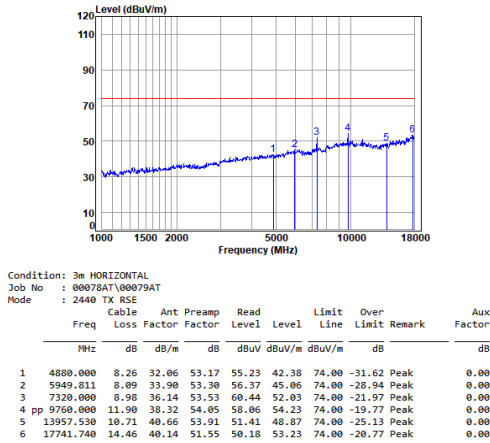
Headset 2.4G SRD_1M_TX_CH_19_Horizontal-Peak
