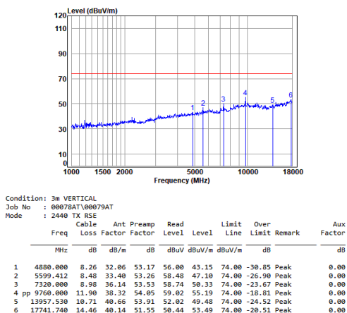
Headset 2.4G SRD_2M_TX_CH_19_Vertical-Peak
