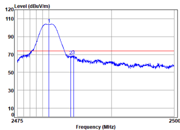
Headset 2.4G SRD_2M_TX_CH_39_Vertical-Peak
