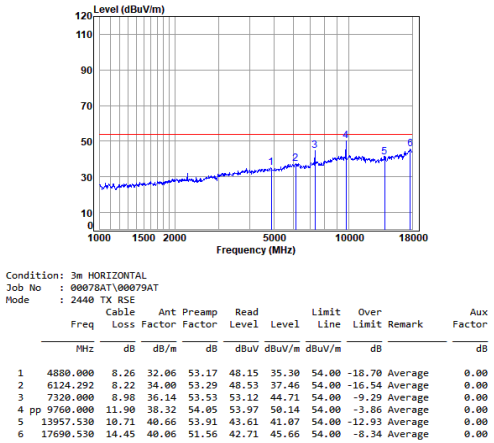
Headset 2.4G SRD_1M_TX_CH_19_Horizontal-Avg
