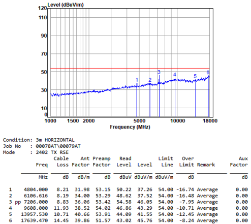
Headset 2.4G SRD_2M_TX_CH_00_Horizontal-Avg
