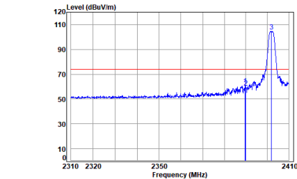
Headset 2.4G SRD_2M_TX_CH_00_Vertical-Peak
