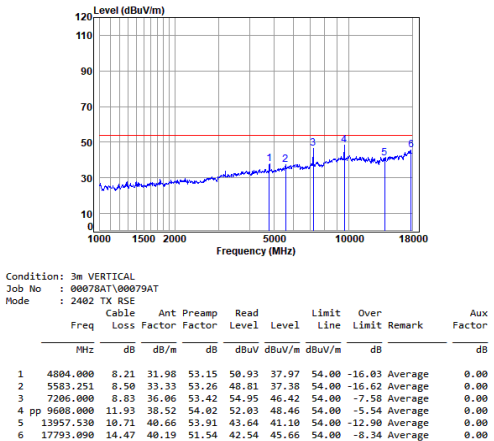
Headset 2.4G SRD_2M_TX_CH_00_Vertical-Avg
