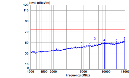
Headset 2.4G SRD_1M_TX_CH_00_Horizontal-Peak
