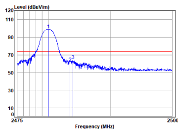
Headset 2.4G SRD_1M_TX_CH_39_Horizontal-Peak
