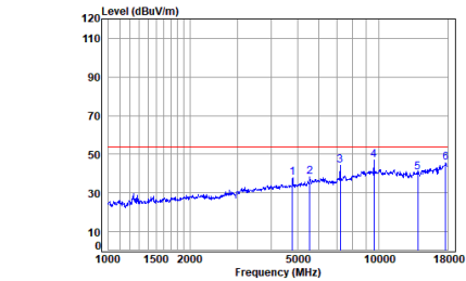
Headset 2.4G SRD_1M_TX_CH_00_Vertical-Avg
