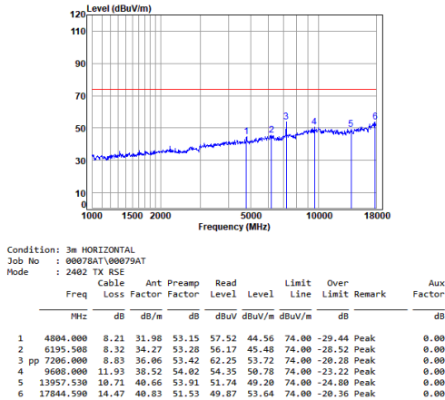
Headset 2.4G SRD_2M_TX_CH_00_Horizontal-Peak
