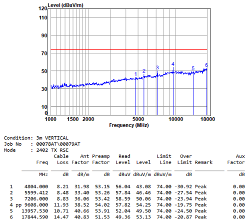
Headset 2.4G SRD_2M_TX_CH_00_Vertical-Peak
