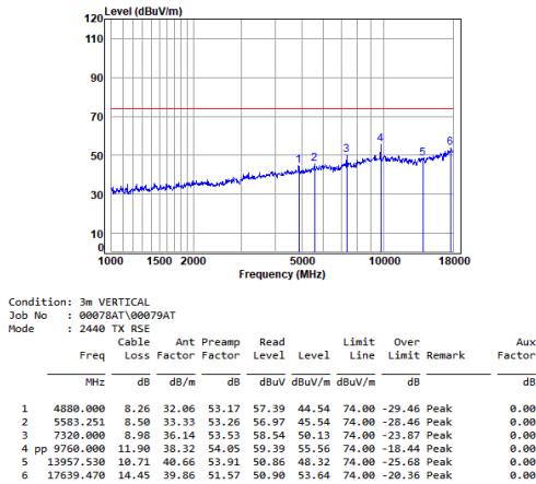
Headset 2.4G SRD_1M_TX_CH_19_Vertical-Peak
