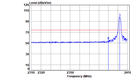
Headset 2.4G SRD_1M_TX_CH_00_Horizontal-Peak
