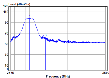
Headset 2.4G SRD_2M_TX_CH_39_Horizontal-Peak
