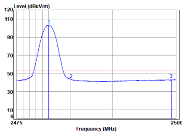
Headset 2.4G SRD_1M_TX_CH_39_Vertical-Avg
