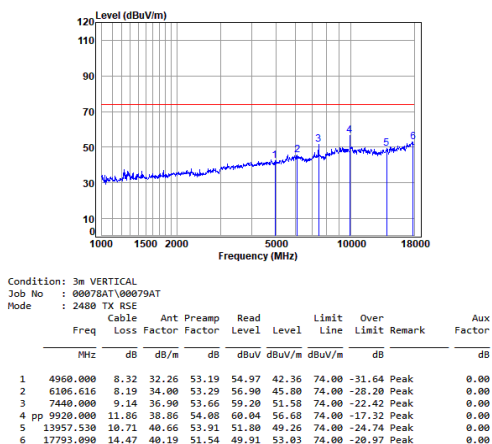
Headset 2.4G SRD_1M_TX_CH_39_Vertical-Peak
