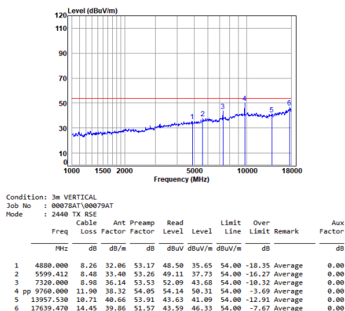
Headset 2.4G SRD_2M_TX_CH_19_Vertical-Avg
