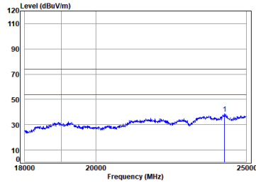
Headset 2.4G SRD_1M_TX_CH_19_Horizontal-Peak
