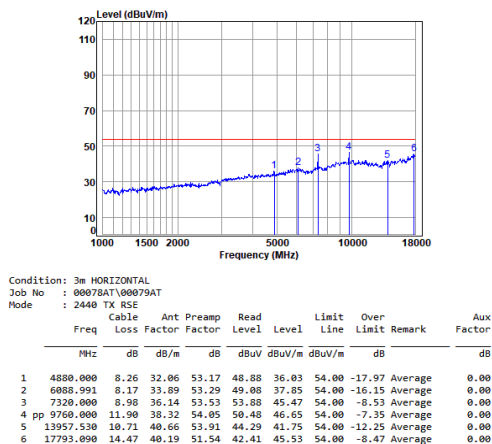
Headset 2.4G SRD_2M_TX_CH_19_Horizontal-Avg
