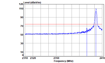
Headset 2.4G SRD_1M_TX_CH_00_Vertical-Peak
