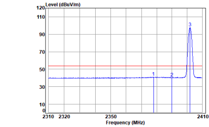
Headset 2.4G SRD_1M_TX_CH_00_Horizontal-Avg
