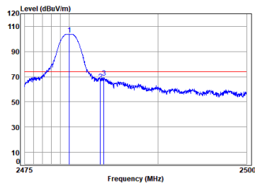
Headset 2.4G SRD_1M_TX_CH_39_Vertical-Peak
