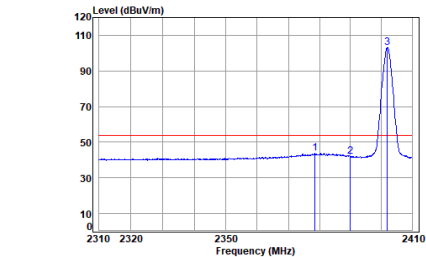
Headset 2.4G SRD_2M_TX_CH_00_Vertical-Avg
