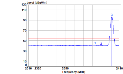
Headset 2.4G SRD_2M_TX_CH_00_Horizontal-Avg
