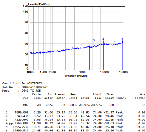
Headset 2.4G SRD_2M_TX_CH_19_Horizontal-Peak
