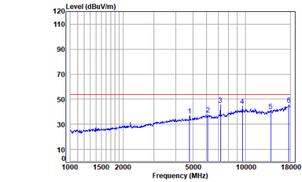
Headset 2.4G SRD_1M_TX_CH_00_Horizontal-Avg
