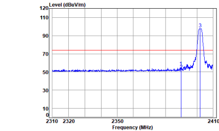
Headset 2.4G SRD_2M_TX_CH_00_Horizontal-Peak
