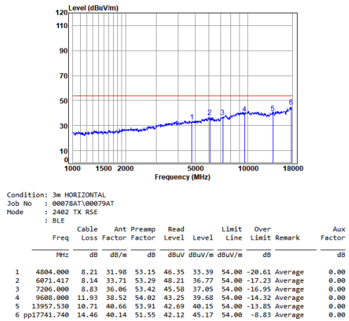
Headset BLE_2M_TX_CH_00_Horizontal-Avg
