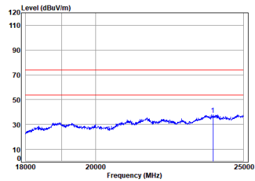
Headset BLE_1M_TX_CH_19_Vertical-Peak
