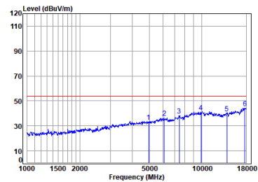
Headset BLE_1M_TX_CH_39_Vertical-Avg
