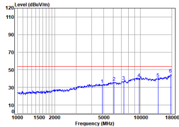
Headset BLE_1M_TX_CH_19_Vertical-Avg
