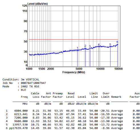
Headset BLE_1M_TX_CH_00_Vertical-Avg
