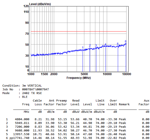
Headset BLE_1M_TX_CH_00_Vertical-Peak
