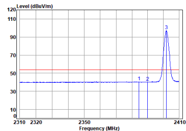
Headset BLE_2M_TX_CH_00_Vertical-Avg
