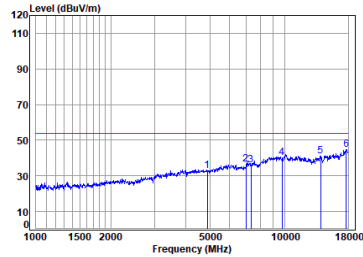
Headset BLE_1M_TX_CH_19_Horizontal-Avg
