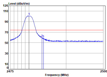
Headset BLE_1M_TX_CH_39_Vertical-Peak
