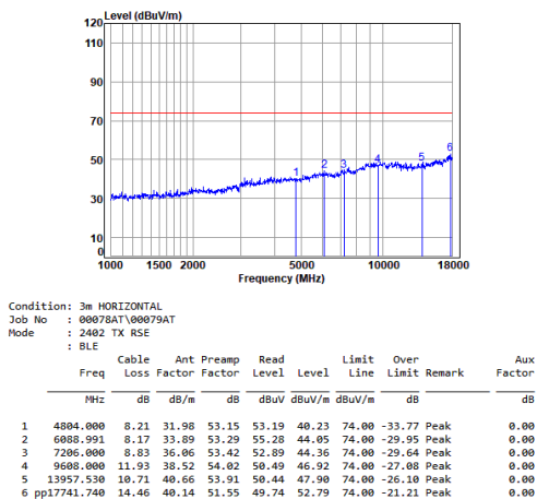
Headset BLE_1M_TX_CH_00_Horizontal-Peak
