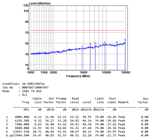
Headset BLE_2M_TX_CH_00_Horizontal-Peak
