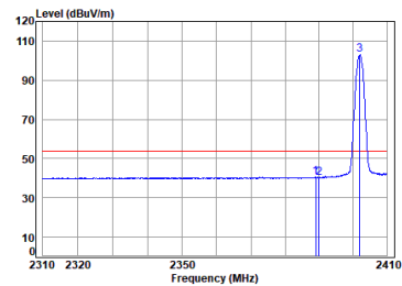
Headset BLE_1M_TX_CH_00_Horizontal-Avg
