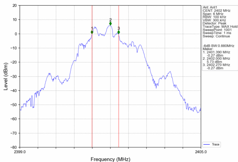
2M_LCH_2402MHz_Ant1_NTNV
