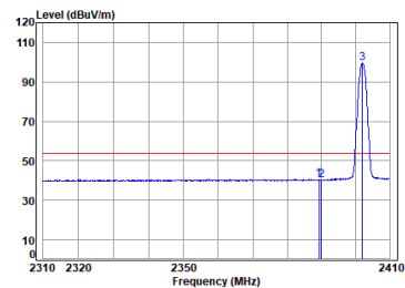
Headset BLE_1M_TX_CH_00_Vertical-Avg
