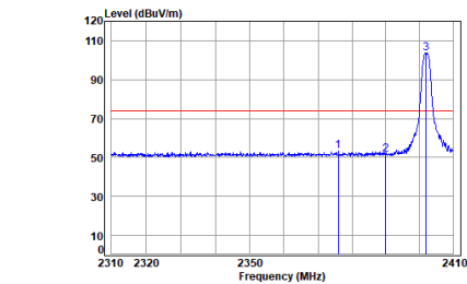
Headset BLE_1M_TX_CH_00_Horizontal-Peak
