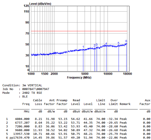
Headset BLE_2M_TX_CH_00_Vertical-Peak
