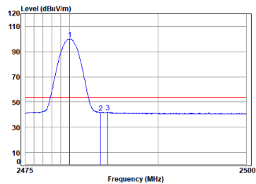
Headset BLE_1M_TX_CH_39_Vertical-Avg
