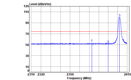
Headset BLE_1M_TX_CH_00_Vertical-Peak
