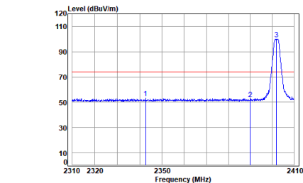
Headset BLE_2M_TX_CH_00_Vertical-Peak
