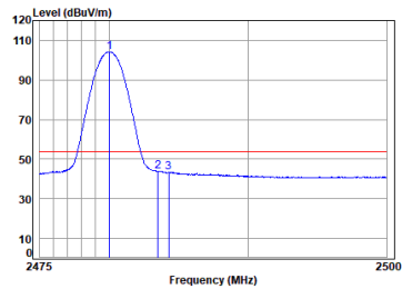
Headset BLE_1M_TX_CH_39_Horizontal-Avg
