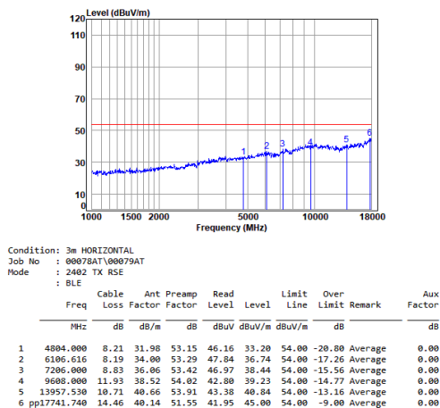
Headset BLE_1M_TX_CH_00_Horizontal-Avg
