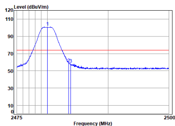
Headset BLE_2M_TX_CH_39_Vertical-Peak
