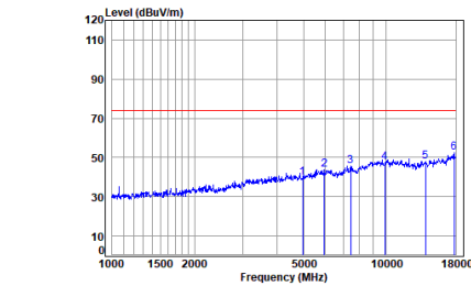
Headset BLE_1M_TX_CH_39_Horizontal-Peak
