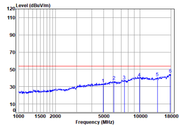
Headset BLE_1M_TX_CH_39_Horizontal-Avg
