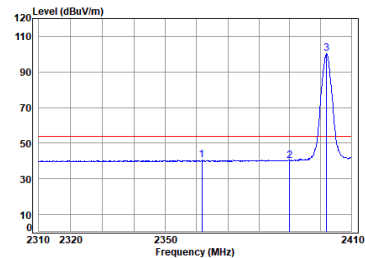
Headset BLE_2M_TX_CH_00_Horizontal-Avg
