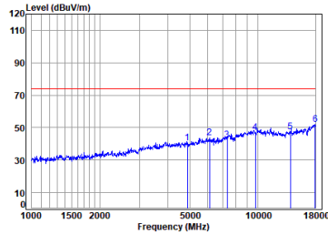
Headset BLE_1M_TX_CH_19_Horizontal-Peak
