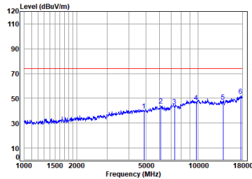
Headset BLE_1M_TX_CH_19_Vertical-Peak
