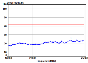
Headset BLE_1M_TX_CH_19_Horizontal-Peak
