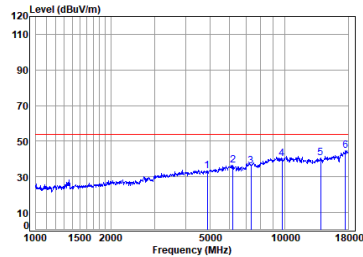
Headset BLE_2M_TX_CH_19_Vertical-Avg
