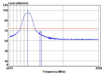
Headset BLE_1M_TX_CH_39_Horizontal-Peak
