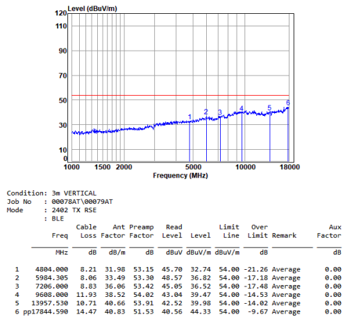
Headset BLE_2M_TX_CH_00_Vertical-Avg
