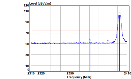
Headset BLE_2M_TX_CH_00_Horizontal-Peak
