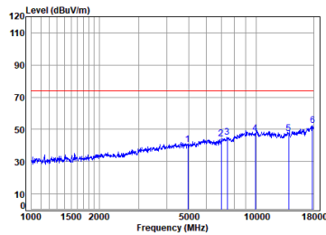
Headset BLE_2M_TX_CH_39_Horizontal-Peak
