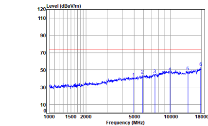
Headset BLE_1M_TX_CH_39_Vertical-Peak
