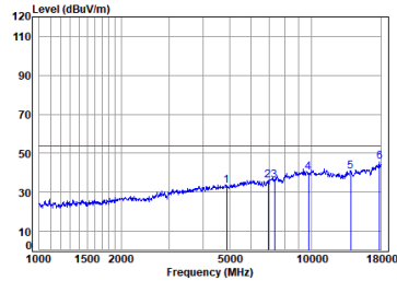
Headset BLE_2M_TX_CH_19_Horizontal-Avg
