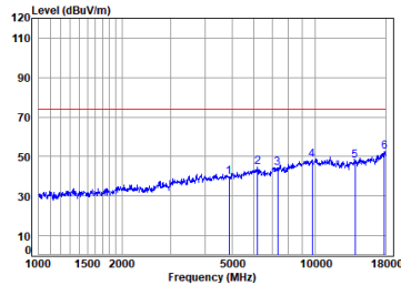
Headset BLE_2M_TX_CH_19_Vertical-Peak
