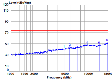
Headset BLE_2M_TX_CH_19_Horizontal-Peak
