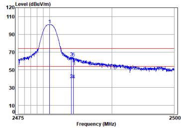
Headset BT_DH5_TX_CH_78_Vertical
