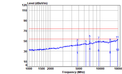
Headset BT_DH5_TX_CH_00_Horizontal
