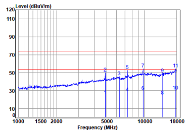
Headset BT_DH5_TX_CH_39_Vertical
