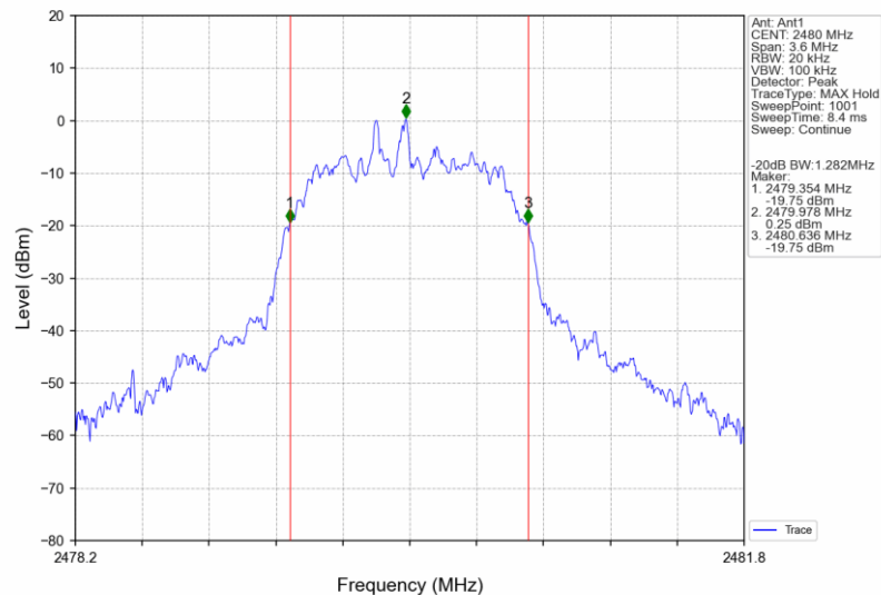
Pi/4DQPSK_2DH5_HCH_2480MHz_Ant1_NTNV
