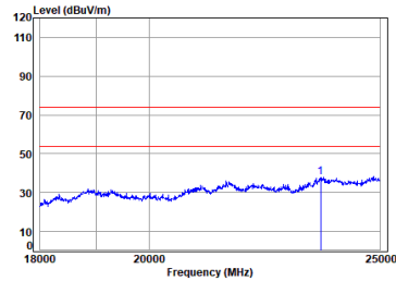
Headset BT_DH5_TX_CH_39_Vertical
