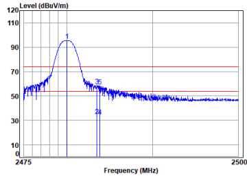
Headset BT_DH5_TX_CH_78_Horizontal
