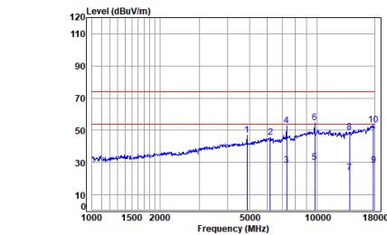
Headset BT_DH5_TX_CH_39_Horizontal
