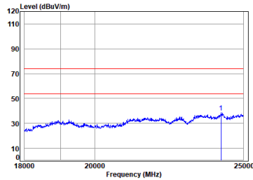
Headset BT_DH5_TX_CH_39_Horizontal
