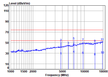
Headset BT_DH5_TX_CH_00_Vertical
