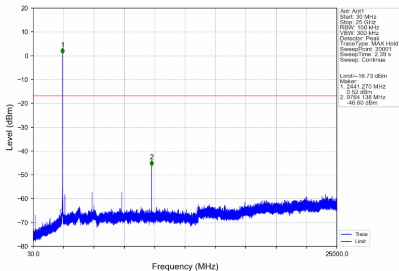
Pi/4DQPSK_2DH5_MCH_2441MHz_Ant1_NTNV
