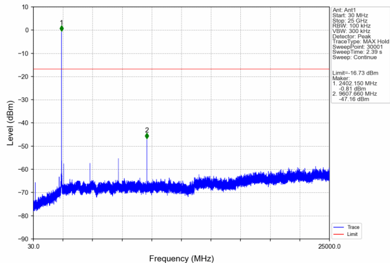
8DPSK_3DH5_LCH_2402MHz_Ant1_NTNV
