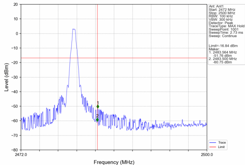
GFSK_DH5_HCH_2480MHz_Ant1_NTNV
