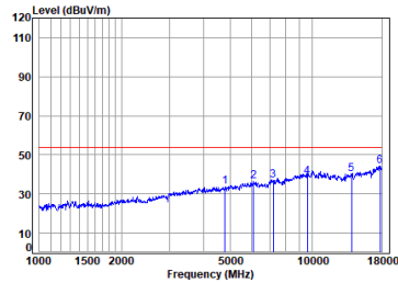
Dongle 2.4SRD_2M_TX_CH_00_Vertical-Avg
