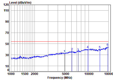
Dongle 2.4SRD_1M_TX_CH_19_Horizontal-Avg
