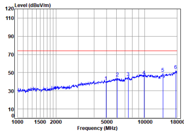
Dongle 2.4SRD_2M_TX_CH_39_Horizontal-Peak
