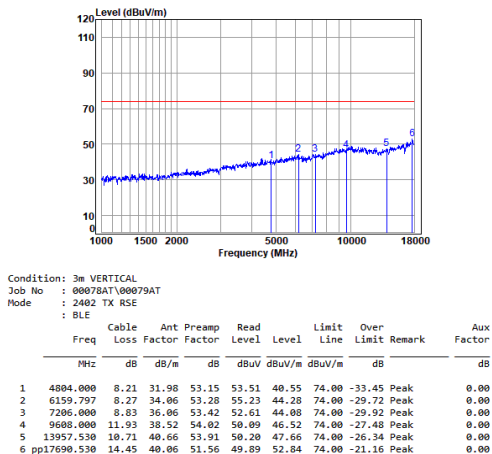
Dongle 2.4SRD_1M_TX_CH_00_Vertical-Peak
