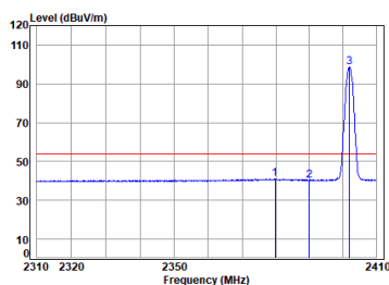
Dongle 2.4G SRD_1M_TX_CH_00_Horizontal-Avg
