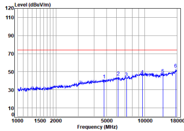
Dongle 2.4SRD_2M_TX_CH_00_Vertical-Peak
