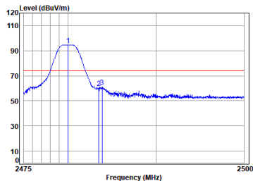
Dongle 2.4G SRD_2M_TX_CH_39_Vertical-Peak
