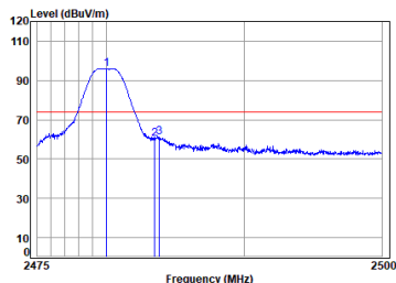
Dongle 2.4G SRD_2M_TX_CH_39_Horizontal-Peak
