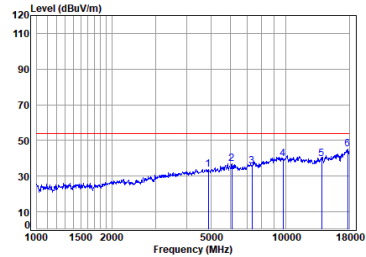
Dongle 2.4SRD2M_TX_CH_19_Horizontal-Avg
