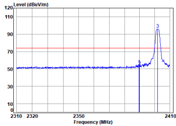
Dongle 2.4G SRD_2M_TX_CH_00_Vertical-Peak
