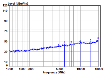
Dongle 2.4SRD_1M_TX_CH_39_Horizontal-Peak
