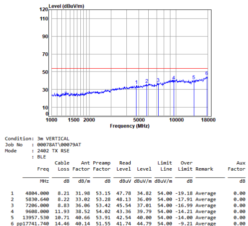
Dongle 2.4SRD_1M_TX_CH_00_Vertical-Avg
