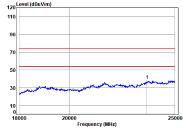
Dongle 2.4SRD_1M_TX_CH_19_Vertical-Peak
