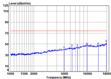
Dongle 2.4SRD_2M_TX_CH_39_Vertical-Peak
