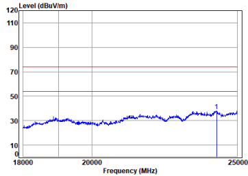
Dongle 2.4SRD_1M_TX_CH_19_Horizontal-Peak
