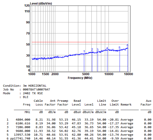
Dongle 2.4SRD_1M_TX_CH_00_Horizontal-Avg
