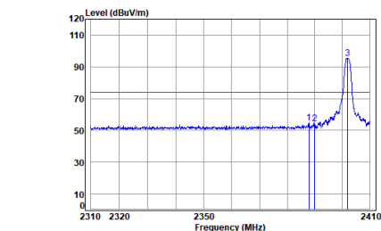
Dongle 2.4G SRD_1M_TX_CH_00_Vertical-Peak
