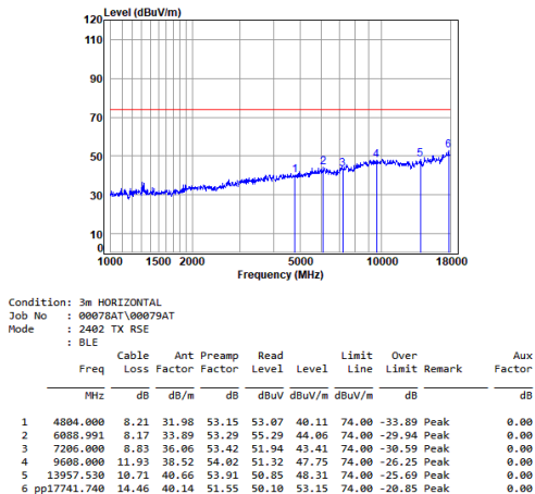
Dongle 2.4SRD_1M_TX_CH_00_Horizontal-Peak
