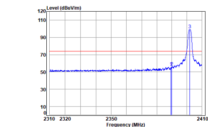
Dongle 2.4G SRD_1M_TX_CH_00_Horizontal-Peak
