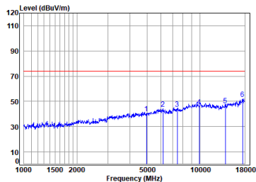
Dongle 2.4SRD_1M_TX_CH_39_Vertical-Peak
