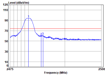
Dongle 2.4G SRD_1M_TX_CH_39_Vertical-Peak
