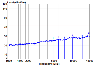
Dongle 2.4SRD_1M_TX_CH_19_Vertical-Peak
