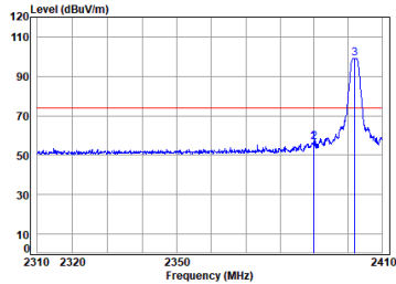
Dongle 2.4G SRD_2M_TX_CH_00_Horizontal-Peak
