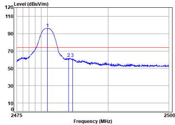
Dongle 2.4G SRD_1M_TX_CH_39_Horizontal-Peak
