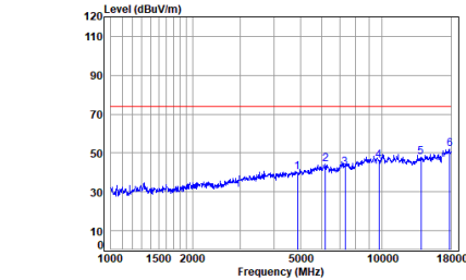
Dongle 2.4SRD_2M_TX_CH_19_Horizontal-Peak
