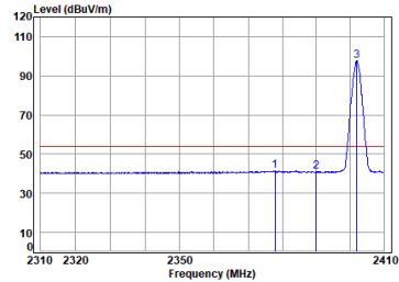
Dongle 2.4G SRD_2M_TX_CH_00_Horizontal-Avg
