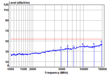
Dongle 2.4SRD_2M_TX_CH_19_Vertical-Avg
