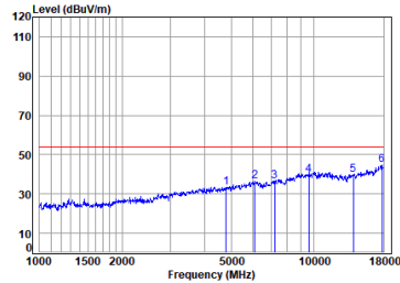
Dongle 2.4SRD_2M_TX_CH_00_Horizontal-Avg
