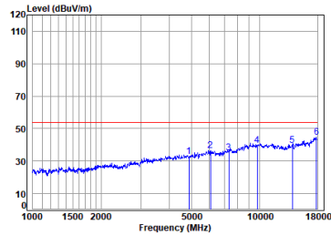
Dongle 2.4SRD_1M_TX_CH_19_Vertical-Avg
