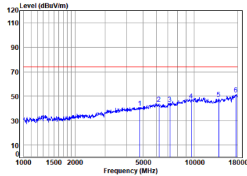
Dongle 2.4SRD_2M_TX_CH_00_Horizontal-Peak
