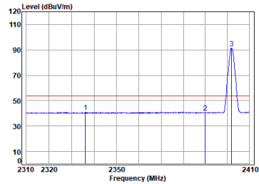
Dongle 2.4G SRD_2M_TX_CH_00_Vertical-Avg
