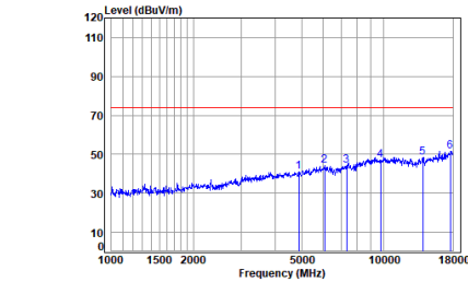
Dongle 2.4SRD_2M_TX_CH_19_Vertical-Peak
