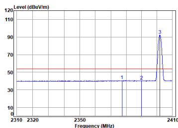
Dongle 2.4G SRD_1M_TX_CH_00_Vertical-Avg
