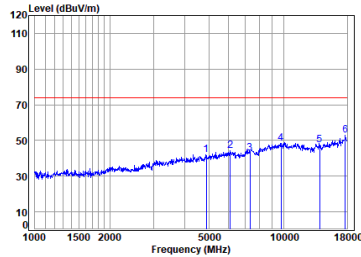
Dongle 2.4SRD_1M_TX_CH_19_Horizontal-Peak
