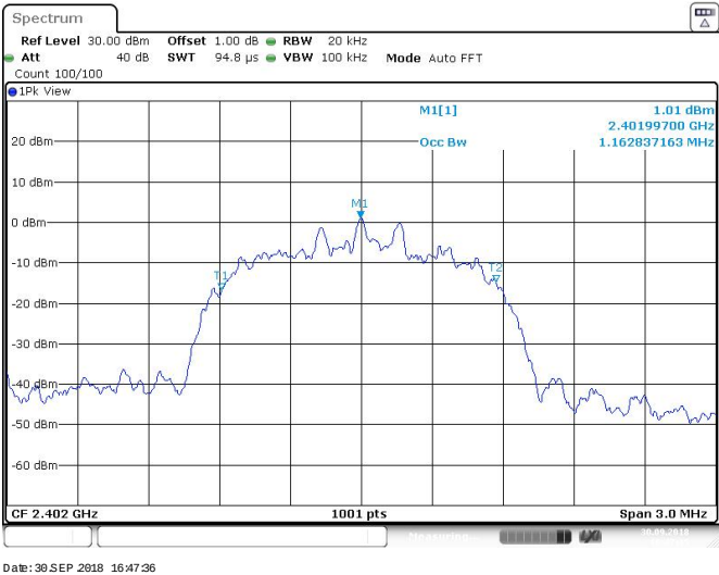
Low channel 2402MHz
