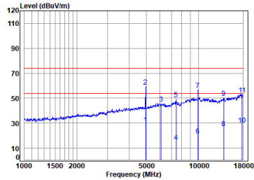
Headset BT_DH5_TX_CH_78_Horizontal
