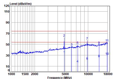
Headset BT_DH5_TX_CH_39_Vertical
