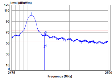
Headset BT_DH5_TX_CH_78_Vertical
