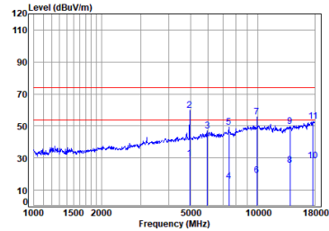
Headset BT_DH5_TX_CH_78_Vertical
