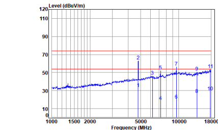
Headset BT_DH5_TX_CH_00_Horizontal
