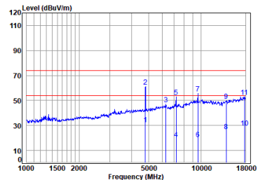
Headset BT_DH5_TX_CH_00_Vertical
