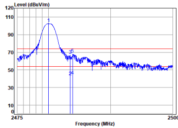
Headset BT_DH5_TX_CH_78_Horizontal
