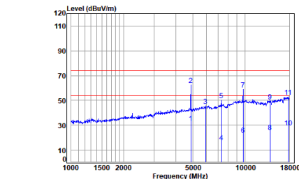
Headset BT_DH5_TX_CH_39_Horizontal
