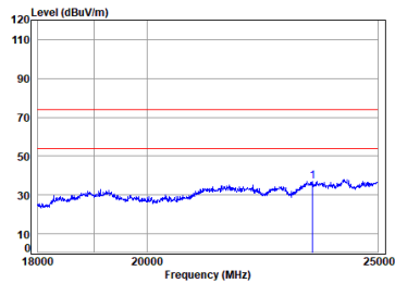
Headset BT_DH5_TX_CH_39_Horizontal
