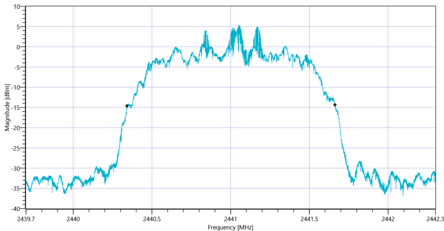
Plot_FCC Part 15.247 Bandwidth 99PCT-20dB ~ BT Classic EDR Pi-4DQPSK 20dB_09122020_151824.png
