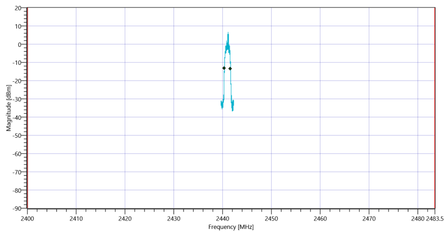
Plot_FCC Part 15.247 Bandwidth 99PCT-20dB ~ BT Classic EDR 8DPSK_09122020_154111.png
