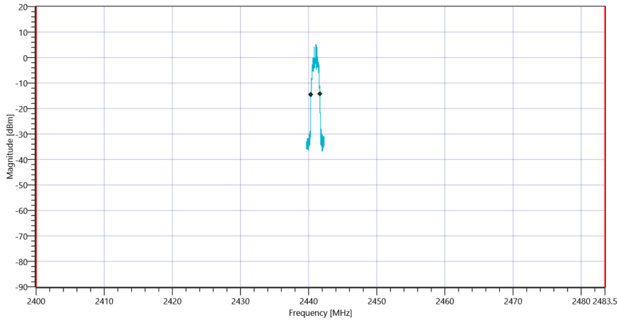
Plot_FCC Part 15.247 Bandwidth 99PCT-20dB ~ BT Classic EDR Pi-4DQPSK_09122020_151827.png
