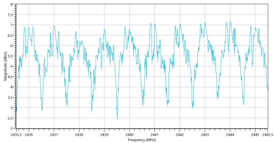
Plot_FCC Part 15.247 Carrier Frequency Separation FHSS ~ BT Classic EDR Pi-4DQPSK_09122020_151700.png
