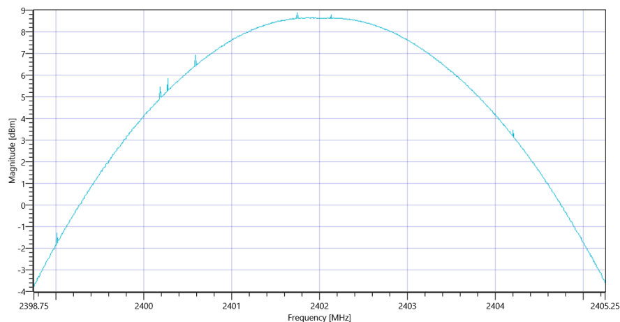
Plot_Common2G4 Peak OP 3MHz-3MHz ~ BT Classic EDR Pi-4DQPSK_09122020_151258.png
