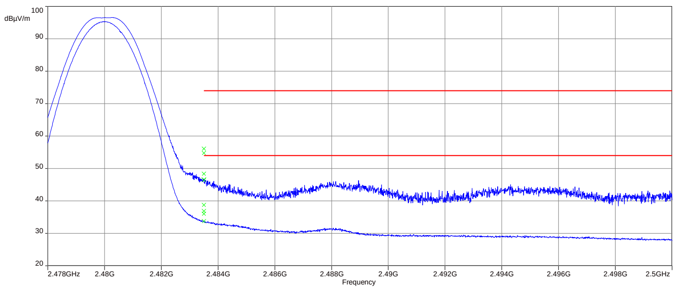
Plot 2: Upper restricted band, 1 Msp
