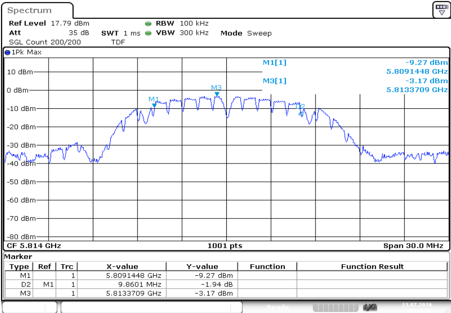
Plot 12: 5814 MHz
