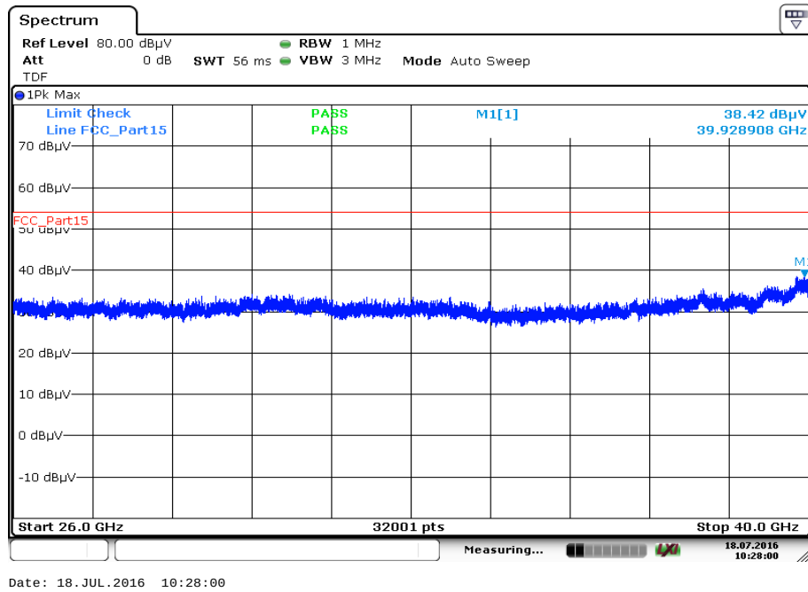
Plot 54: 26 GHz to 40 GHz, 5240 MHz, vertical & horizontal polarization
