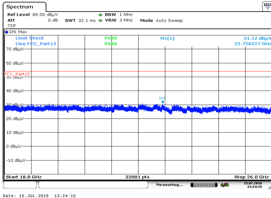
Plot 125: 18 GHz to 26 GHz, 5240 MHz, vertical & horizontal polarization
