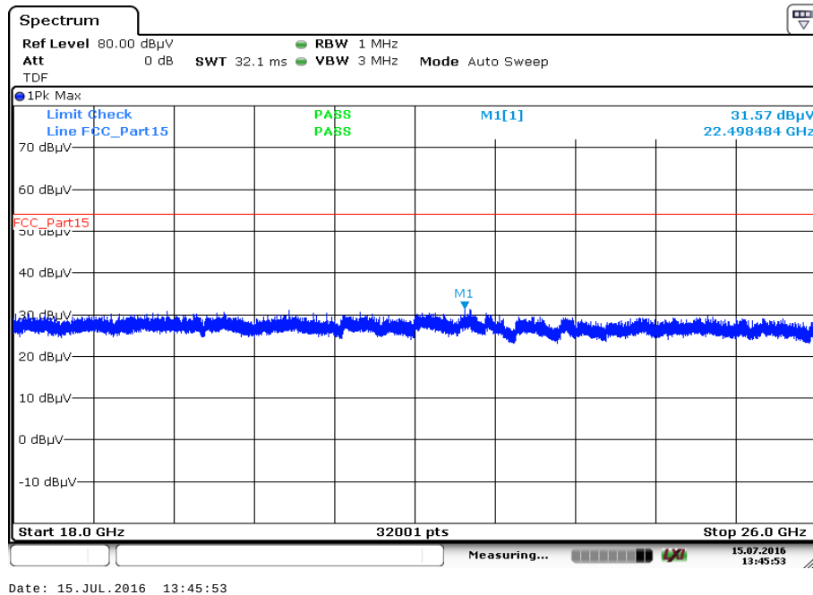
Plot 131: 18 GHz to 26 GHz, 5736 MHz, vertical & horizontal polarization
