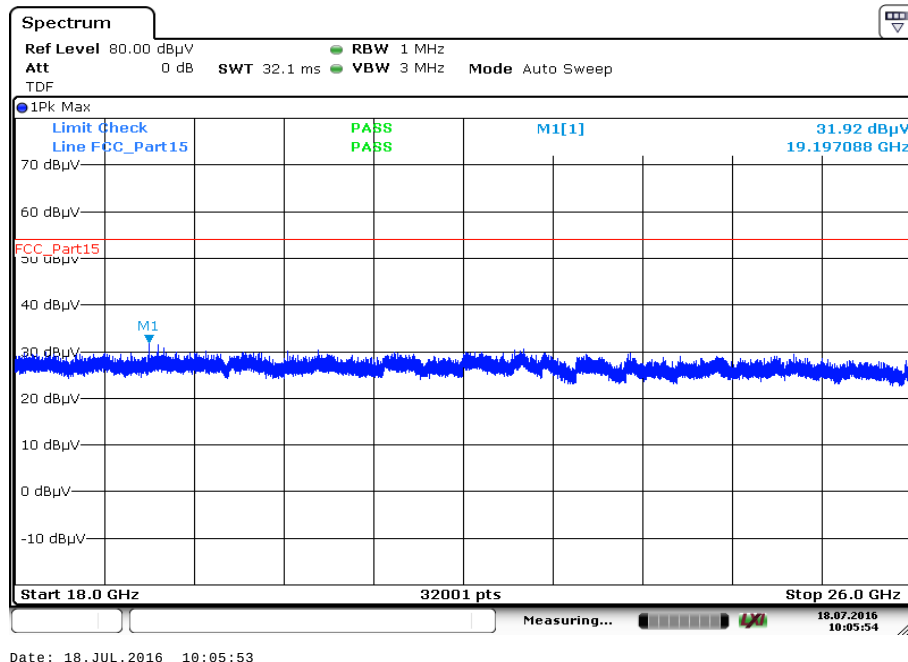
Plot 59: 18 GHz to 26 GHz, 5736 MHz, vertical & horizontal polarization
