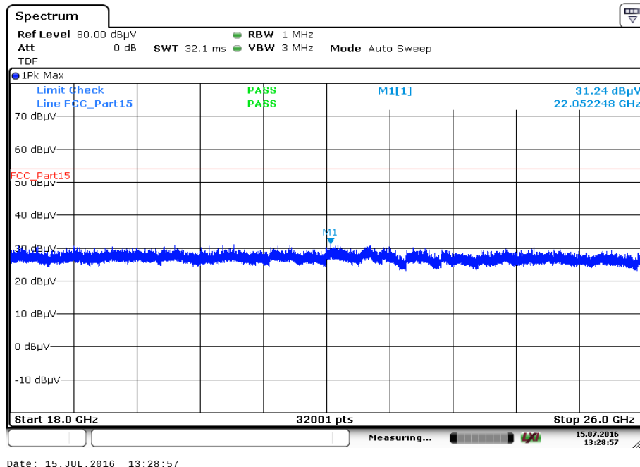
Plot 83: 18 GHz to 26 GHz, 5210 MHz, vertical & horizontal polarization
