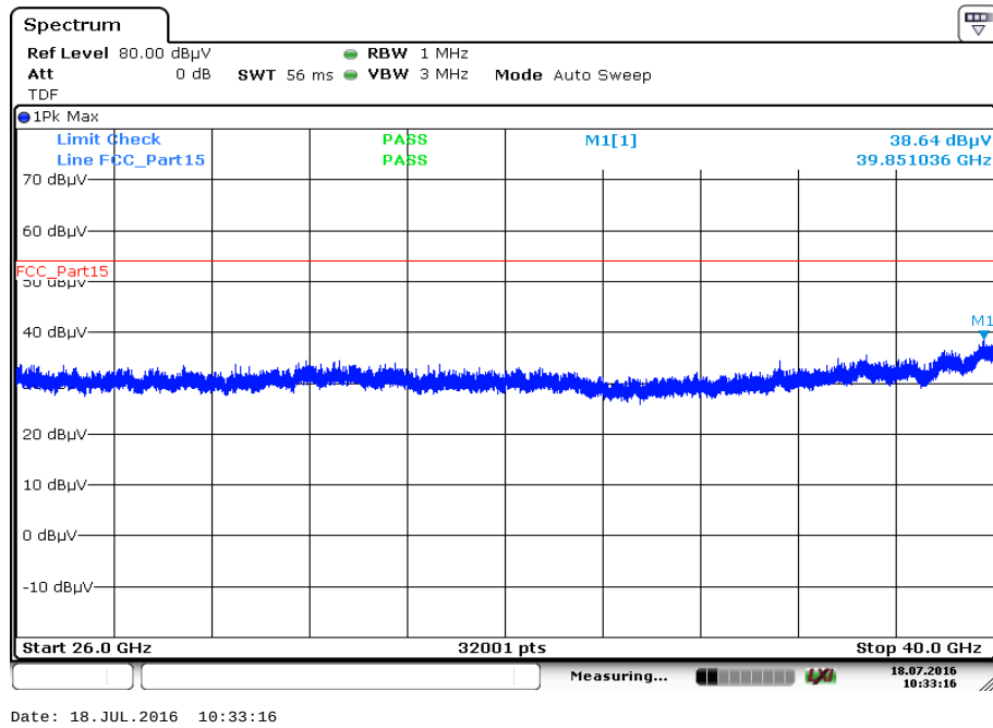
Plot 30: 26 GHz to 40 GHz, 5762 MHz, vertical & horizontal polarization
