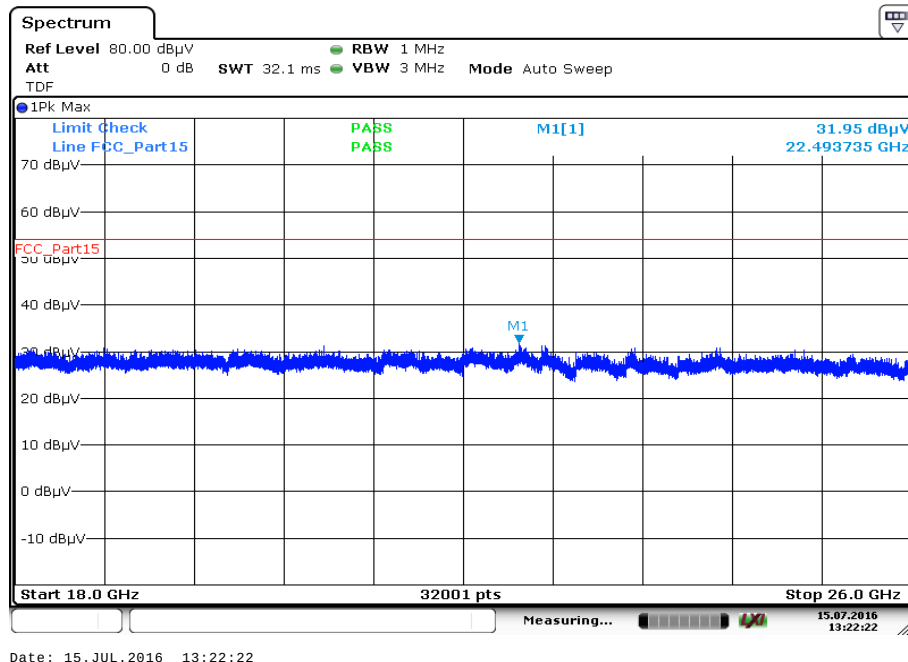
Plot 119: 18 GHz to 26 GHz, 5210 MHz, vertical & horizontal polarization
