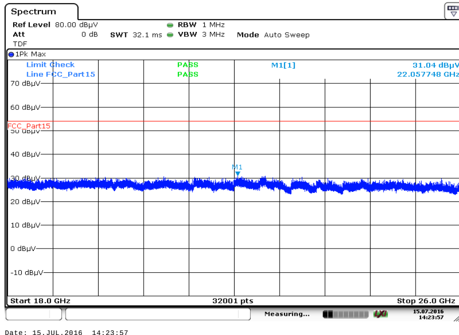
Plot 11: 18 GHz to 26 GHz, 5210 MHz, vertical & horizontal polarization
