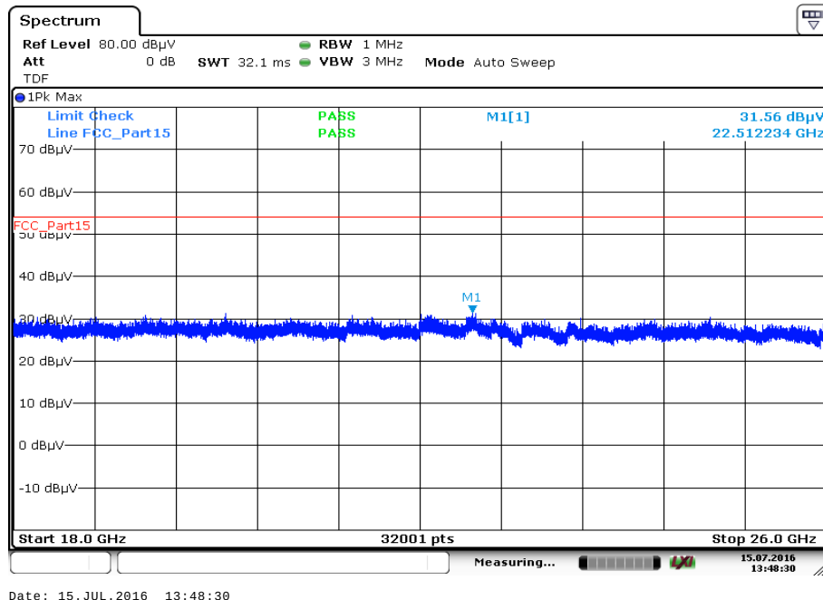
Plot 143: 18 GHz to 26 GHz, 5814 MHz, vertical & horizontal polarization
