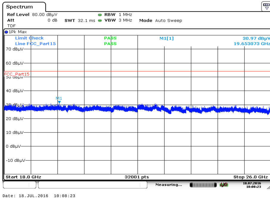
Plot 71: 18 GHz to 26 GHz, 5814 MHz, vertical & horizontal polarization
