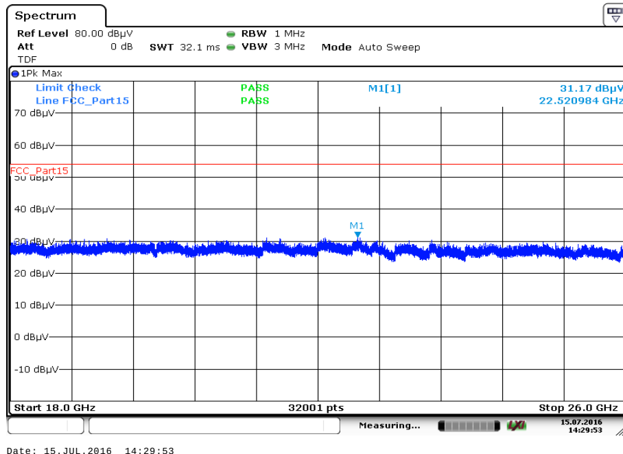
Plot 35: 18 GHz to 26 GHz, 5814 MHz, vertical & horizontal polarization
