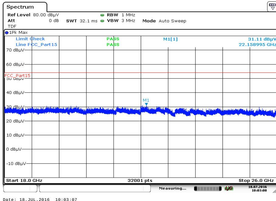
Plot 53: 18 GHz to 26 GHz, 5240 MHz, vertical & horizontal polarization
