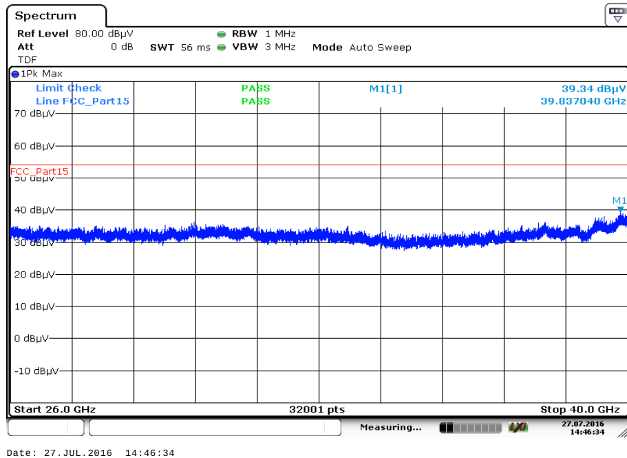
Plot 12: 26 GHz to 40 GHz, vertical & horizontal polarization
