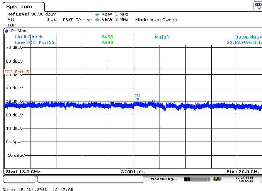
Plot 137: 18 GHz to 26 GHz, 5762 MHz, vertical & horizontal polarization
