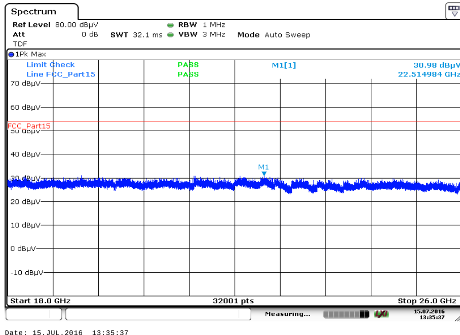
Plot 89: 18 GHz to 26 GHz, 5240 MHz, vertical & horizontal polarization
