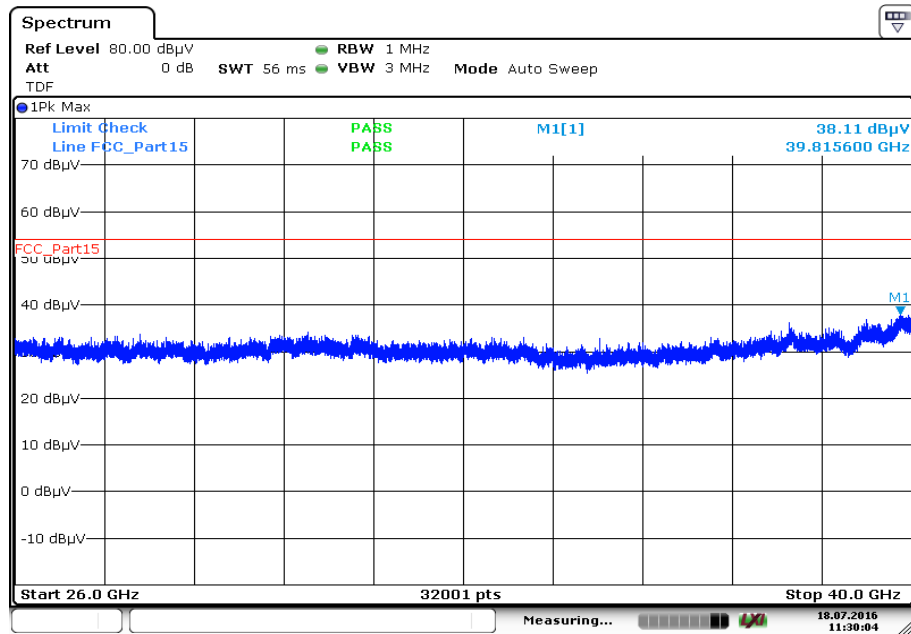
Plot 144: 26 GHz to 40 GHz, 5814 MHz, vertical & horizontal polarization
