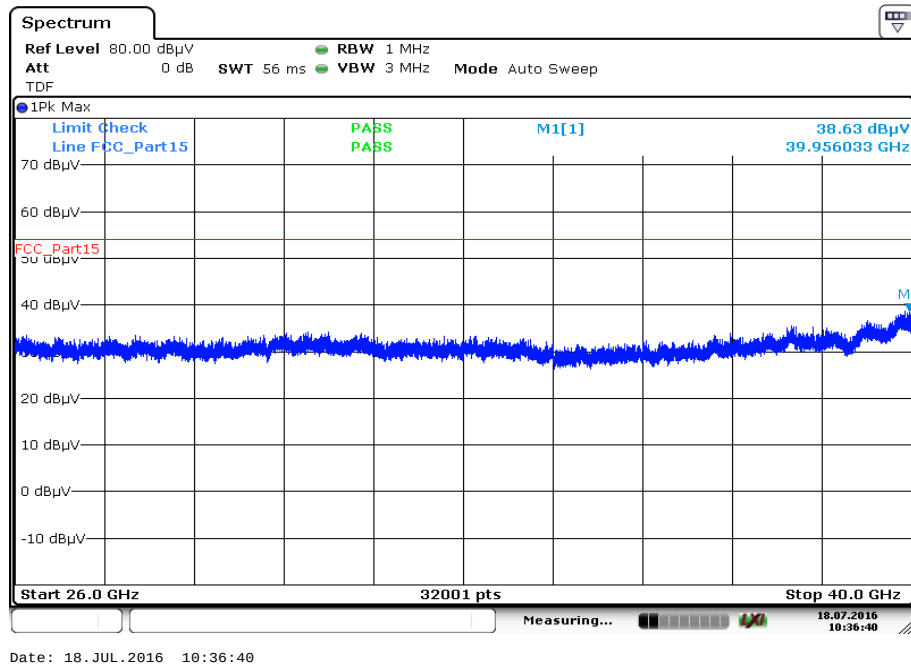
Plot 66: 26 GHz to 40 GHz, 5762 MHz, vertical & horizontal polarization
