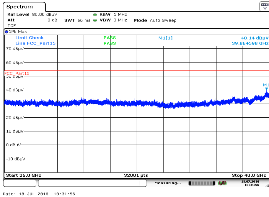
Plot 24: 26 GHz to 40 GHz, 5736 MHz, vertical & horizontal polarization
