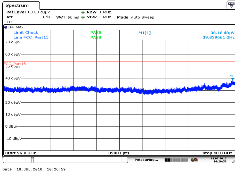
Plot 48: 26 GHz to 40 GHz, 5210 MHz, vertical & horizontal polarization
