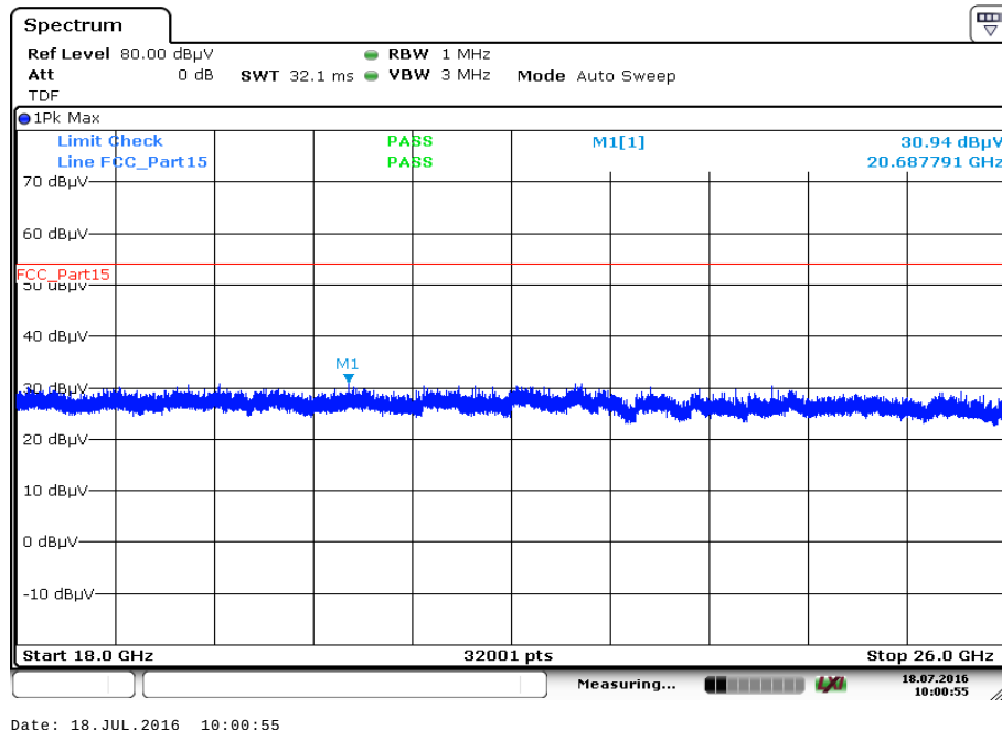
Plot 41: 18 GHz to 26 GHz, 5180 MHz, vertical & horizontal polarization
