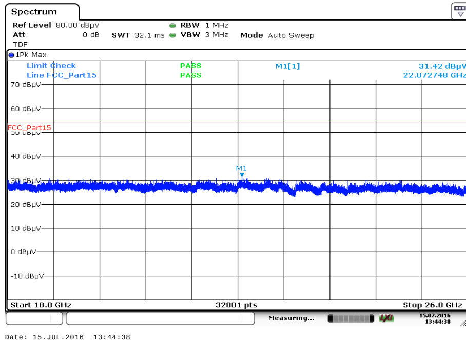
Plot 107: 18 GHz to 26 GHz, 5814 MHz, vertical & horizontal polarization
