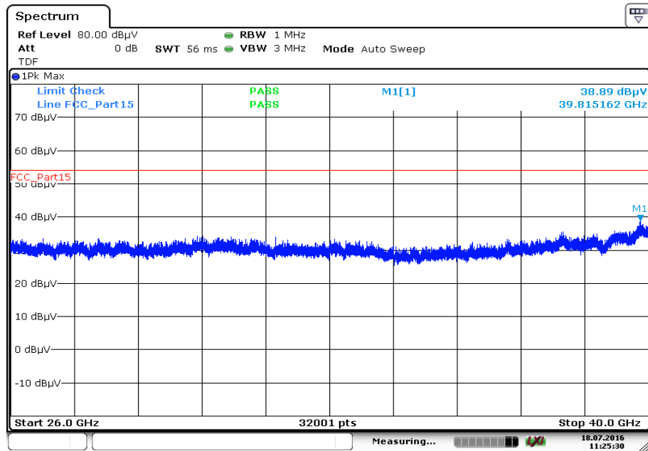
Plot 132: 26 GHz to 40 GHz, 5736 MHz, vertical & horizontal polarization
