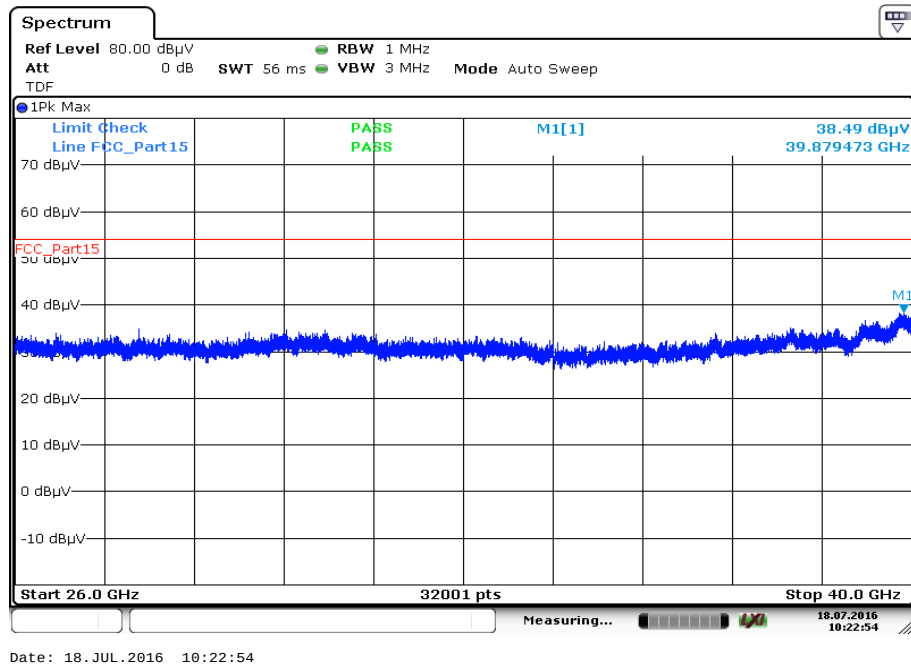
Plot 12: 26 GHz to 40 GHz, 5210 MHz, vertical & horizontal polarization
