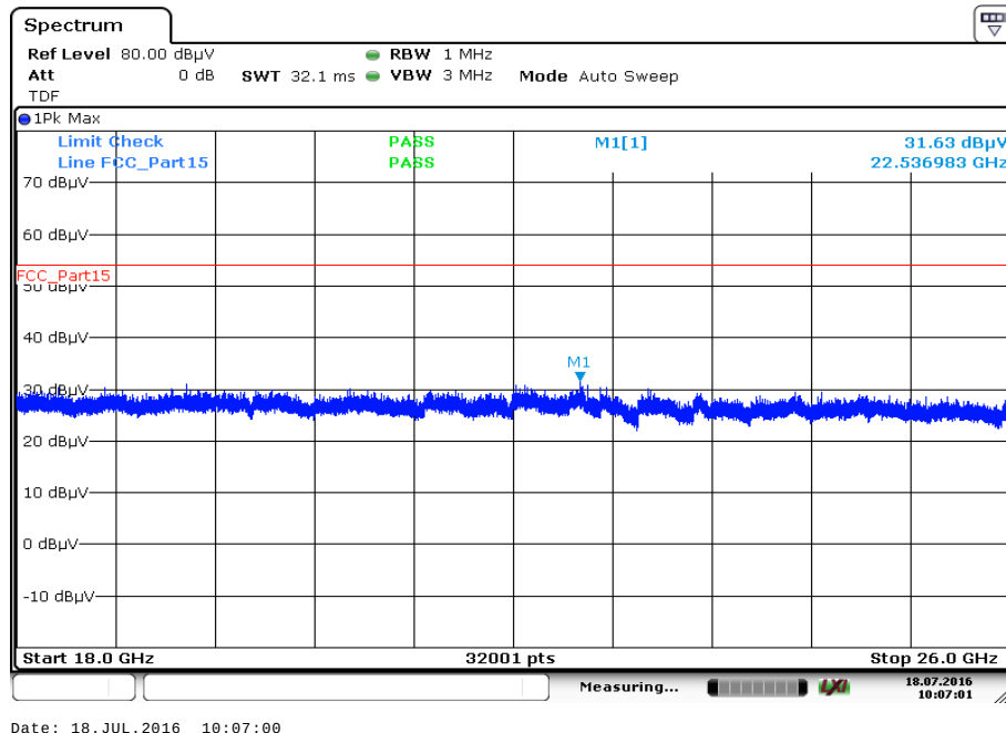
Plot 65: 18 GHz to 26 GHz, 5762 MHz, vertical & horizontal polarization
