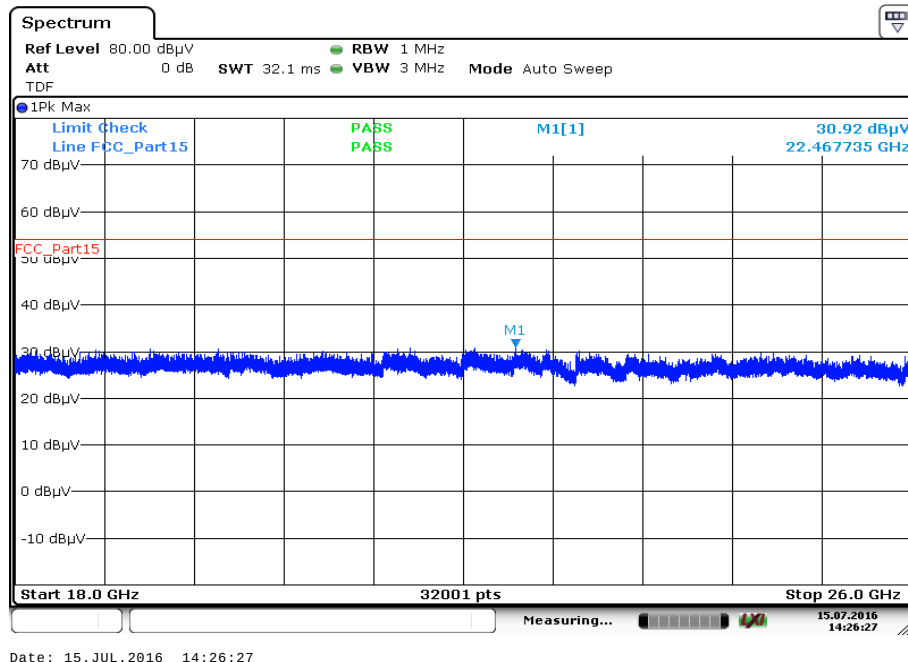
Plot 23: 18 GHz to 26 GHz, 5736 MHz, vertical & horizontal polarization
