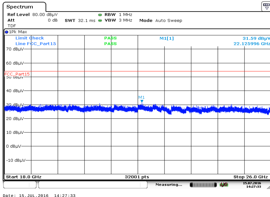
Plot 29: 18 GHz to 26 GHz, 5762 MHz, vertical & horizontal polarization
