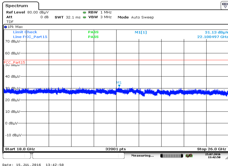
Plot 101: 18 GHz to 26 GHz, 5762 MHz, vertical & horizontal polarization
