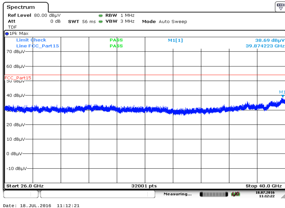
Plot 114: 26 GHz to 40 GHz, 5180 MHz, vertical & horizontal polarization
