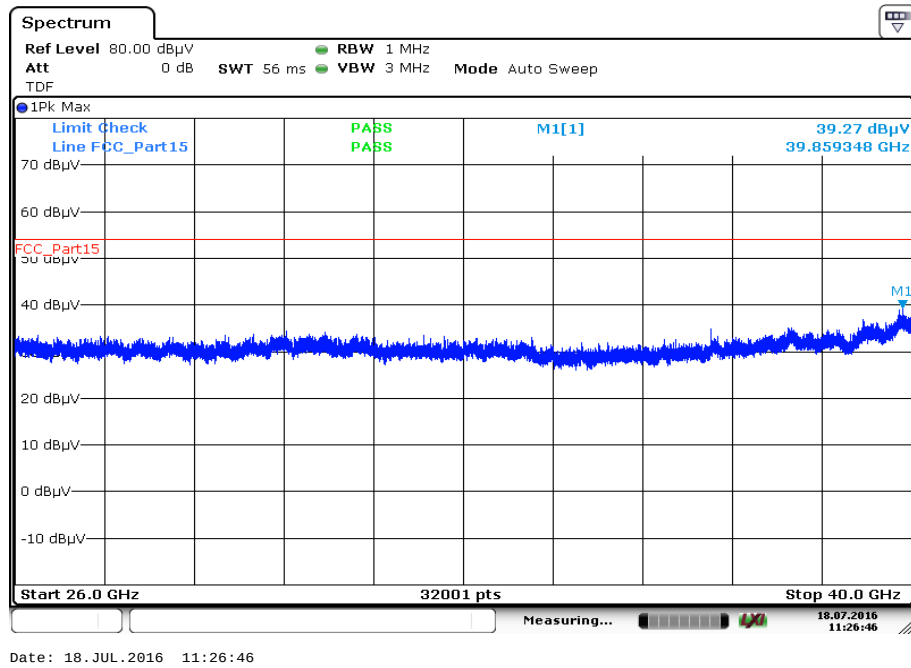
Plot 138: 26 GHz to 40 GHz, 5762 MHz, vertical & horizontal polarization
