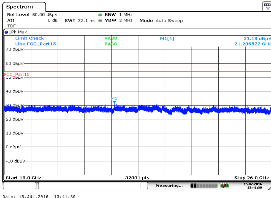
Plot 95: 18 GHz to 26 GHz, 5736 MHz, vertical & horizontal polarization
