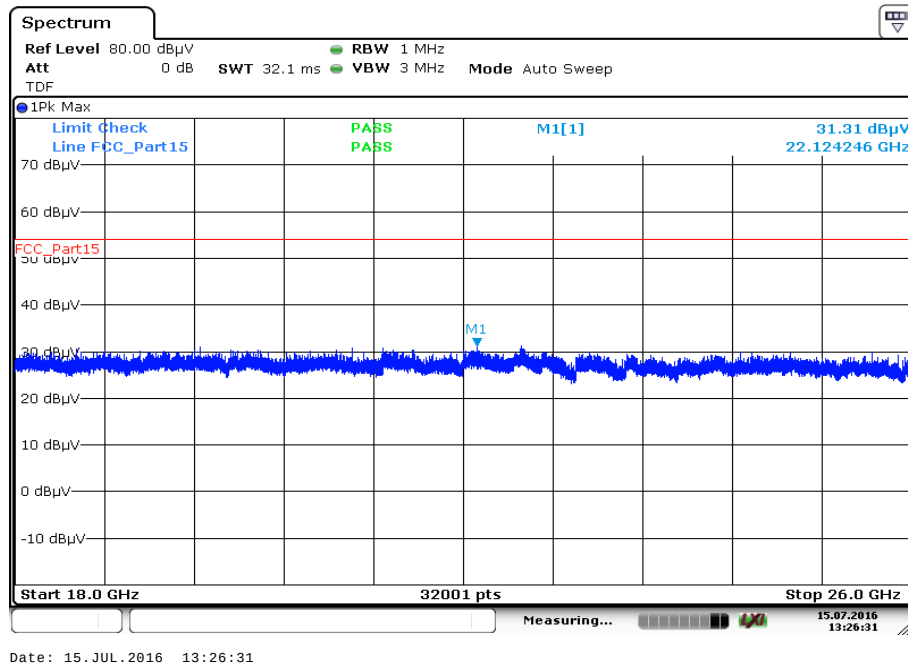
Plot 77: 18 GHz to 26 GHz, 5180 MHz, vertical & horizontal polarization
