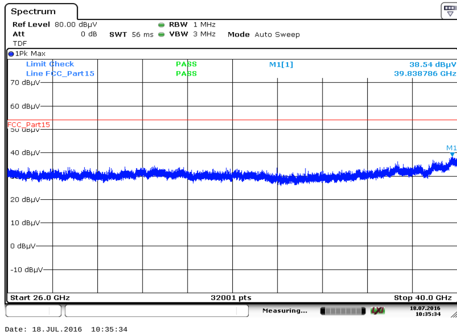
Plot 60: 26 GHz to 40 GHz, 5736 MHz, vertical & horizontal polarization
