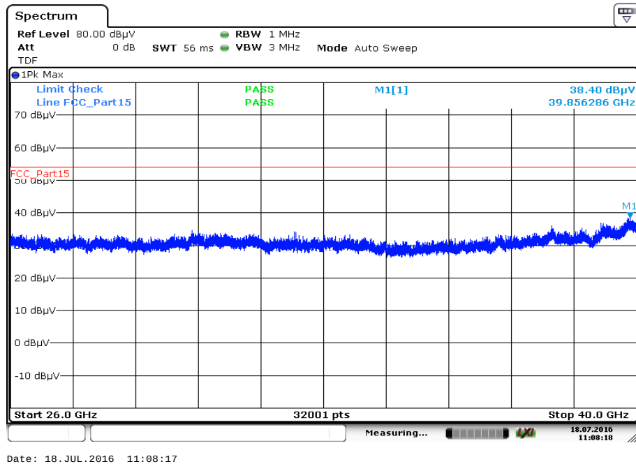
Plot 84: 26 GHz to 40 GHz, 5210 MHz, vertical & horizontal polarization
