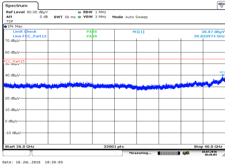
Plot 42: 26 GHz to 40 GHz, 5180 MHz, vertical & horizontal polarization
