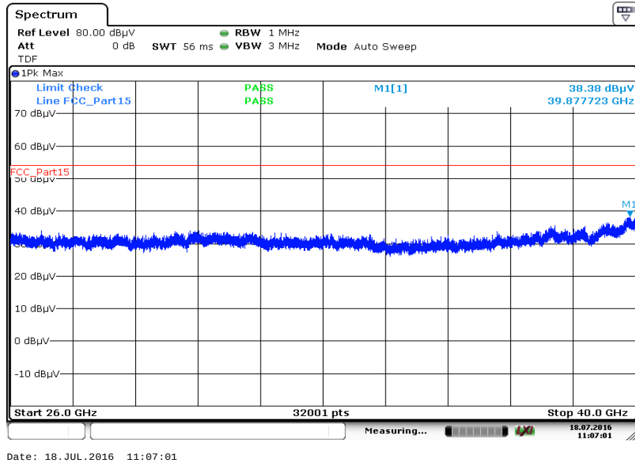
Plot 78: 26 GHz to 40 GHz, 5180 MHz, vertical & horizontal polarization
