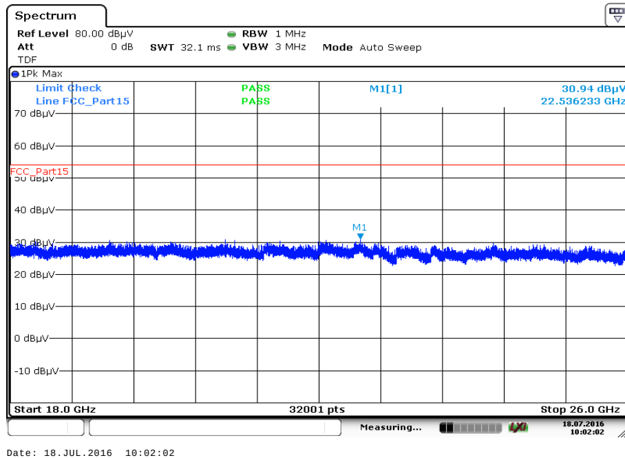
Plot 47: 18 GHz to 26 GHz, 5210 MHz, vertical & horizontal polarization
