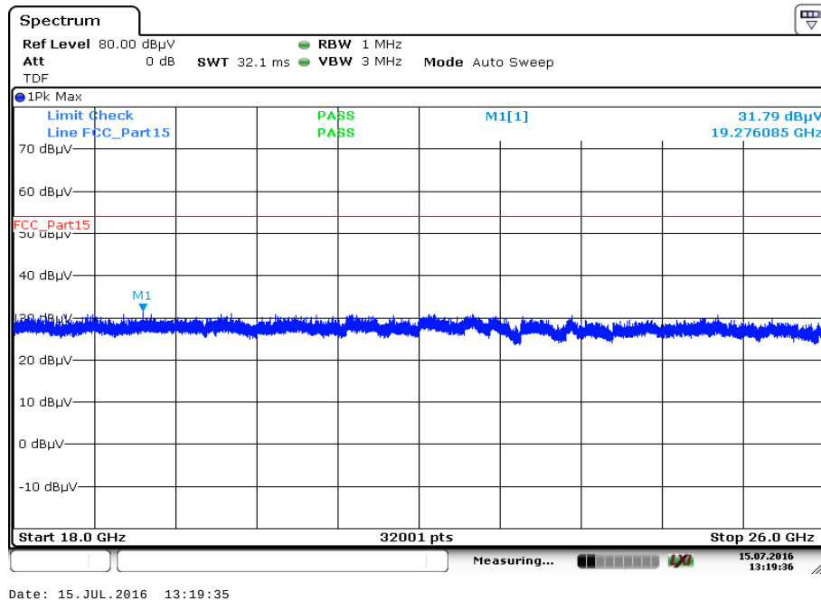
Plot 113: 18 GHz to 26 GHz, 5180 MHz, vertical & horizontal polarization
