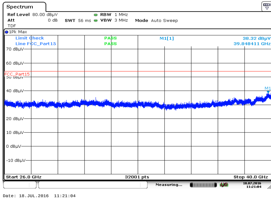
Plot 96: 26 GHz to 40 GHz, 5736 MHz, vertical & horizontal polarization
