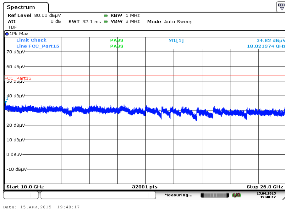
Plot 9: 18 GHz to 26 GHz, 5762 MHz, vertical & horizontal polarization
