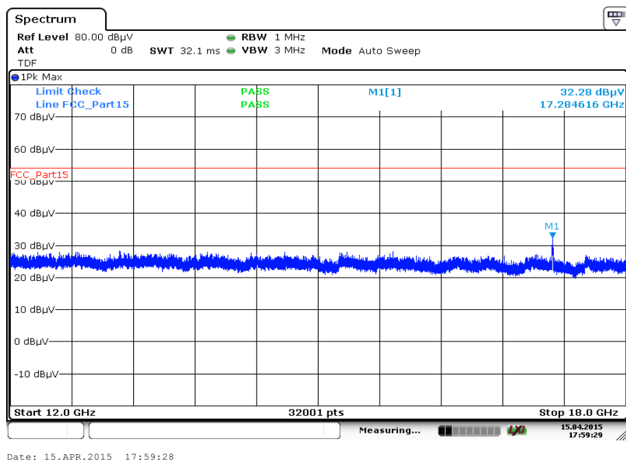
Plot 23: 12 GHz to 18 GHz, 5762 MHz, vertical & horizontal polarization
