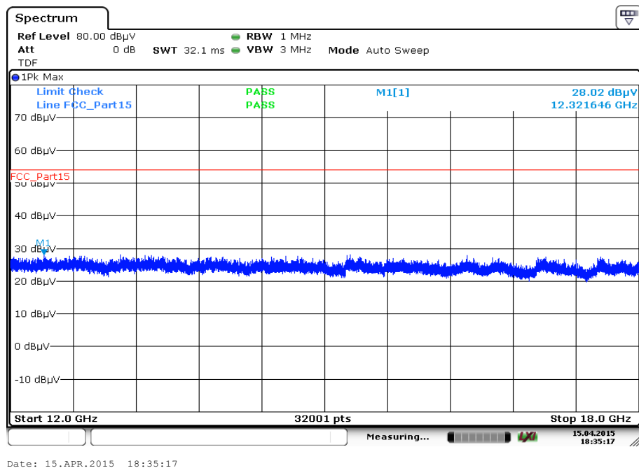
Plot 3: 12 GHz to 18 GHz, 5210 MHz, vertical & horizontal polarization
