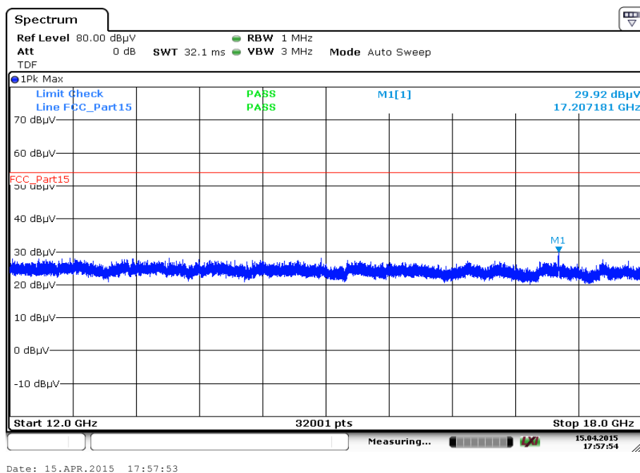
Plot 18: 12 GHz to 18 GHz, 5736 MHz, vertical & horizontal polarization
