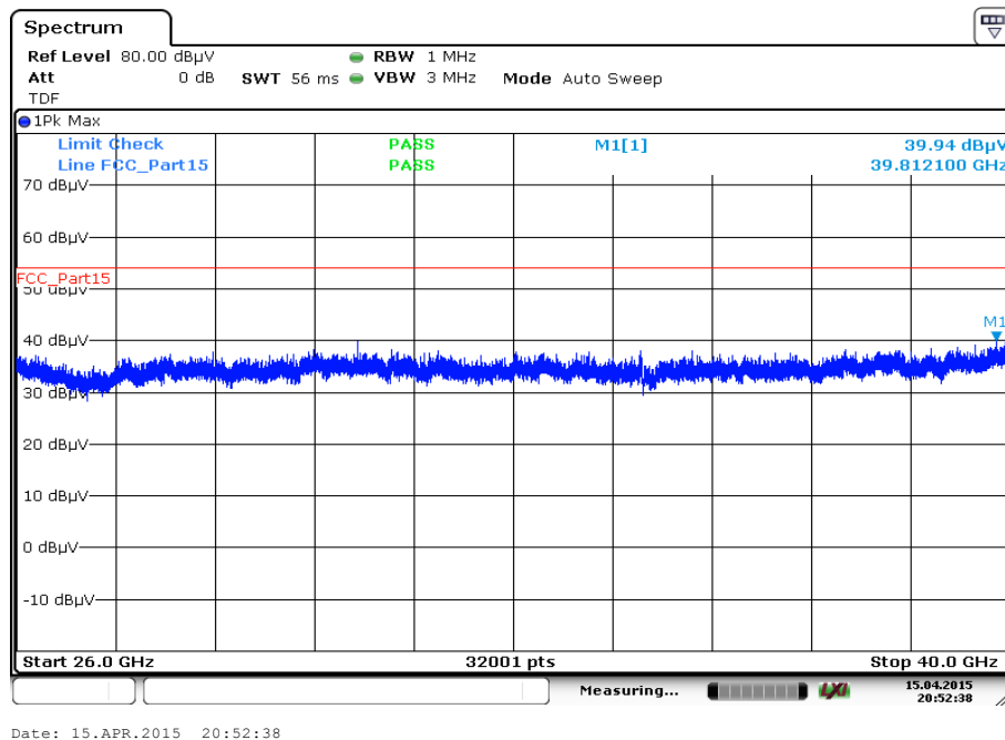
Plot 10: 26 GHz to 40 GHz, 5762 MHz, vertical & horizontal polarization
