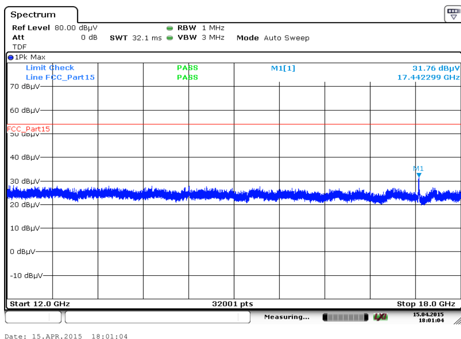
Plot 28: 12 GHz to 18 GHz, 5814 MHz, vertical & horizontal polarization
