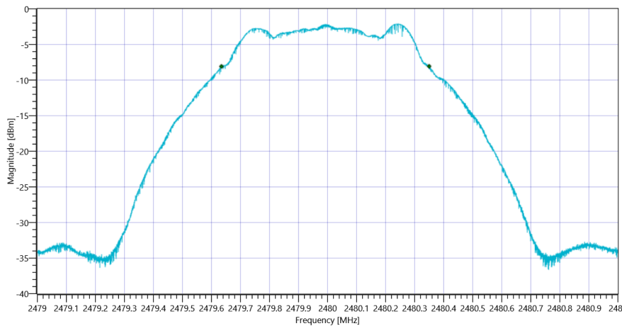
Plot_FCC Part 15.247 Maximum Peak Conducted Output Power DTS ~ BT LE 1 Msps DTS BW_28092021_150454.png
