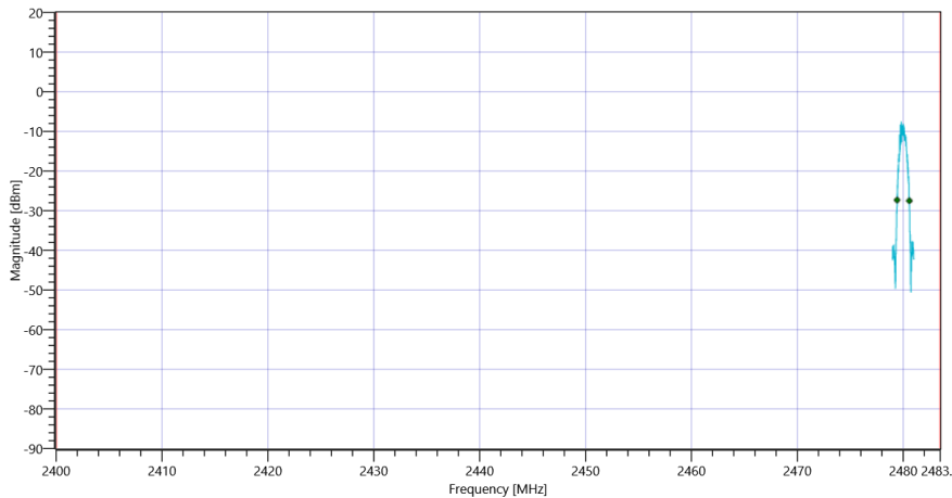
Plot_FCC Part 15.247 Bandwidth 99PCT-20dB ~ BT LE 1 Msps_28092021_150725.png
