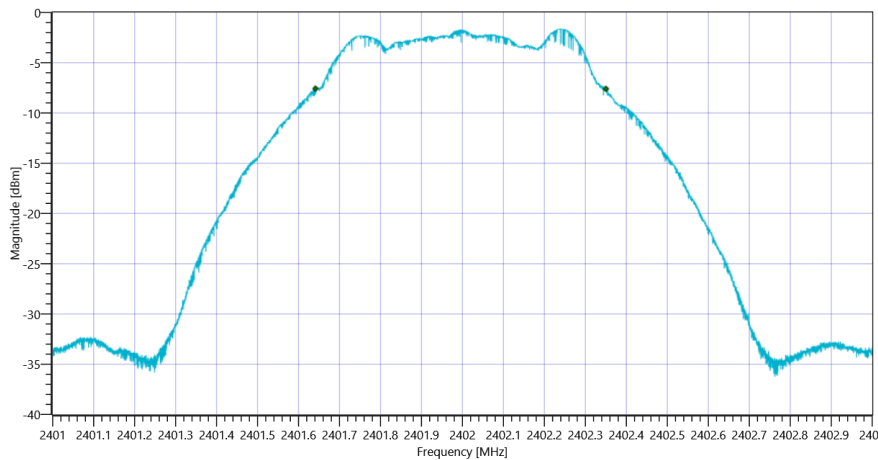
Plot_FCC Part 15.247 Maximum Peak Conducted Output Power DTS ~ BT LE 1 Msps DTS BW_28092021_140604.png
