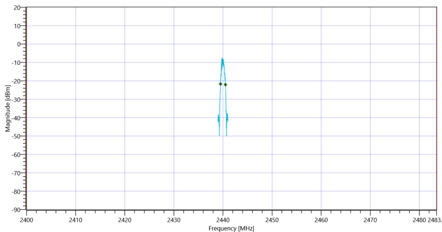
Plot_FCC Part 15.247 Bandwidth 99PCT-20dB ~ BT LE 1 Msps 28092021_142456.png
