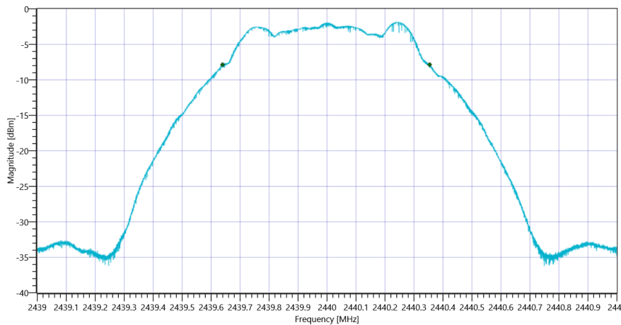
Plot_FCC Part 15.247 Maximum Peak Conducted Output Power DTS ~ BT LE 1 Msps DTS BW_28092021_142239.png
