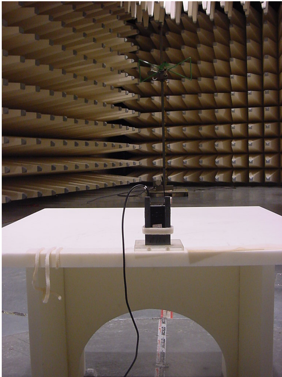
Photo 2: (Radiated Emission)
