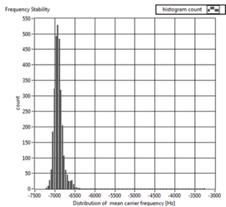
Histogram of Carrier Frequency Stability
