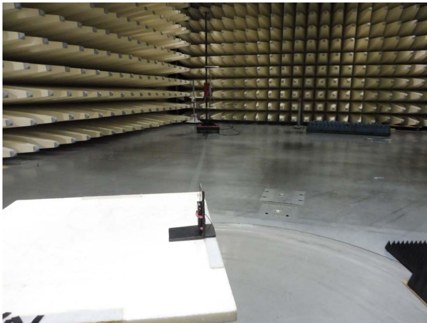
Photo 2: Radiated Emission
