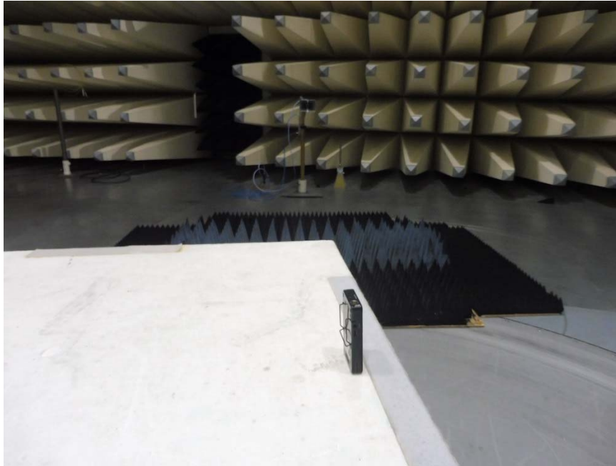
Photo 1: Radiated Emission
