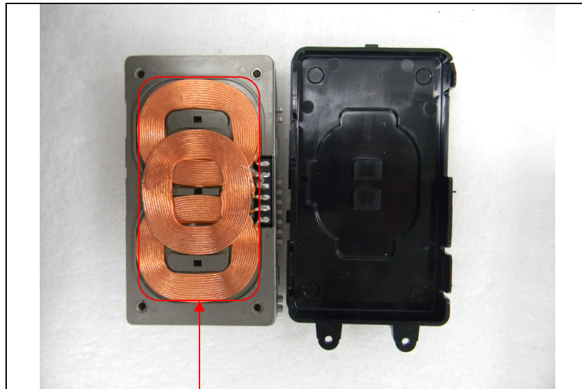
Loop Coil Antenna
