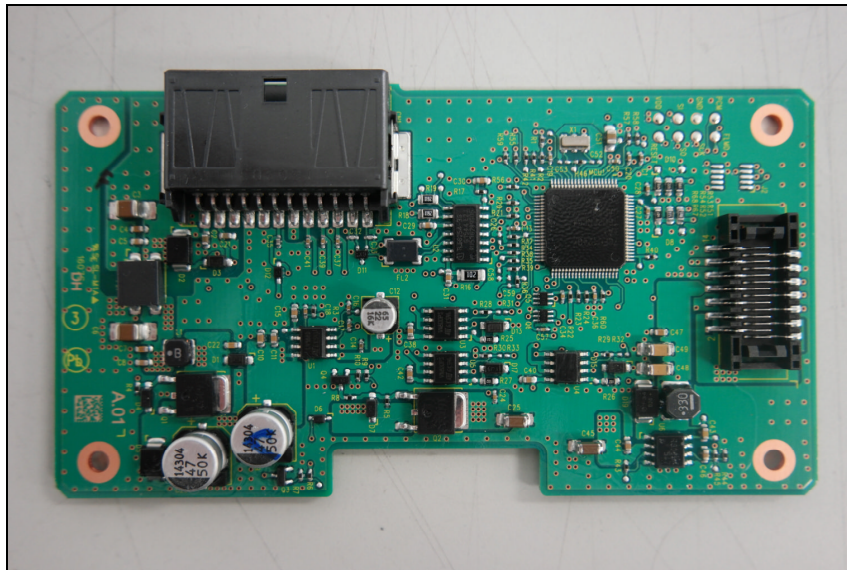
Top view of PCB1
