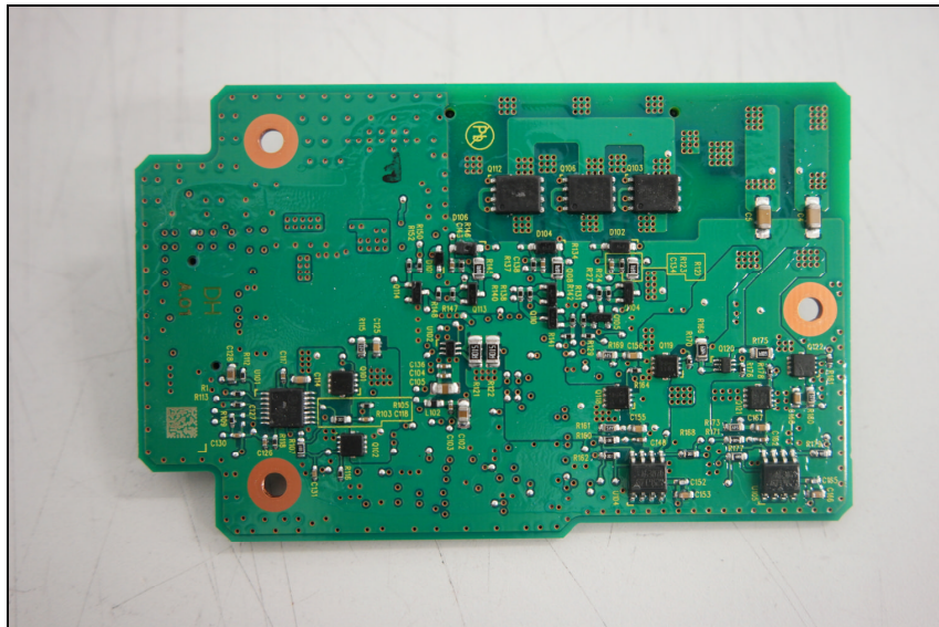
Bottom view of PCB2
