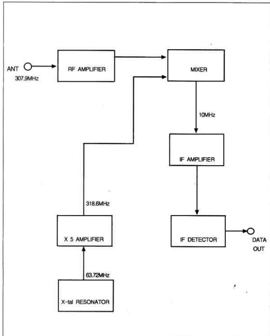
figure 8.1 WMF-R13 Block diagram
