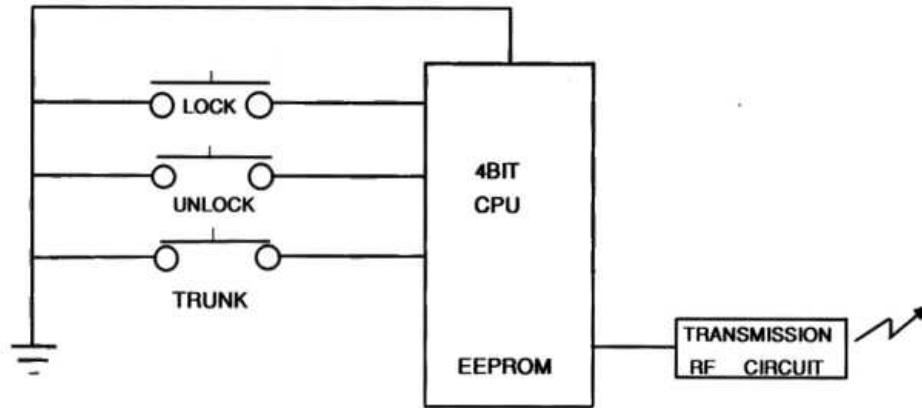
figure 3.1 block diagram of the transmitter
