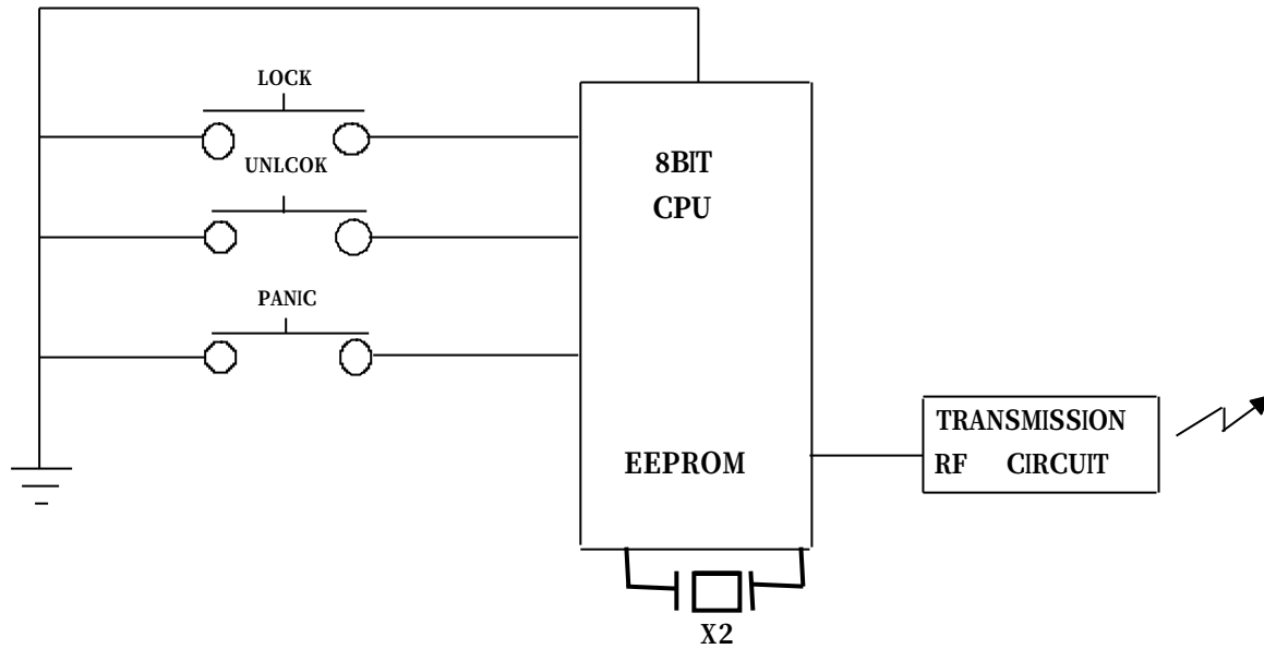
figure . block diagram of the transmitter
