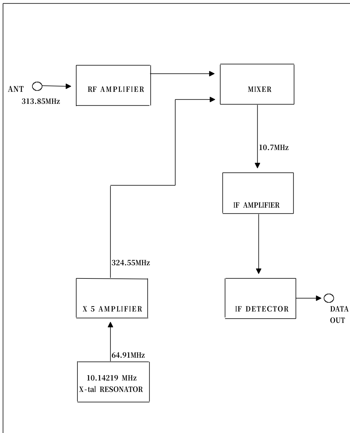
figure 8.1 G8X-21RX Block diagram
