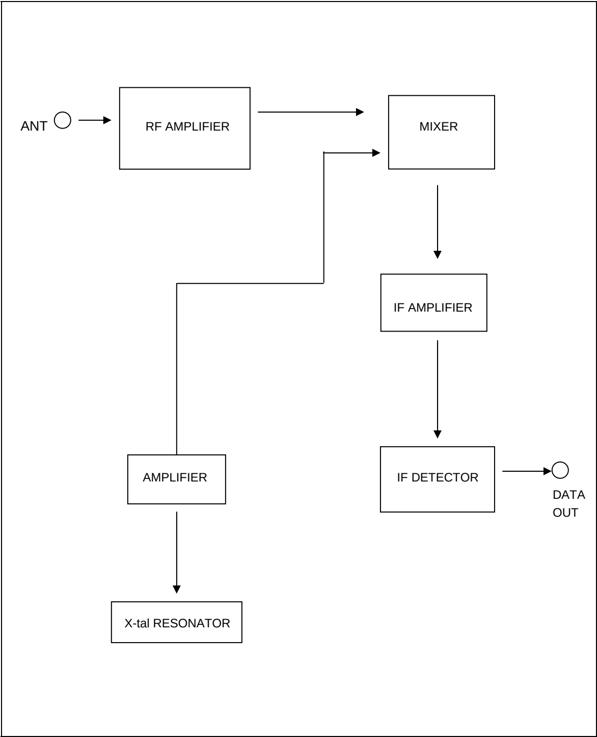
figure 8.1 G8X-21RX1AM Block diagram
