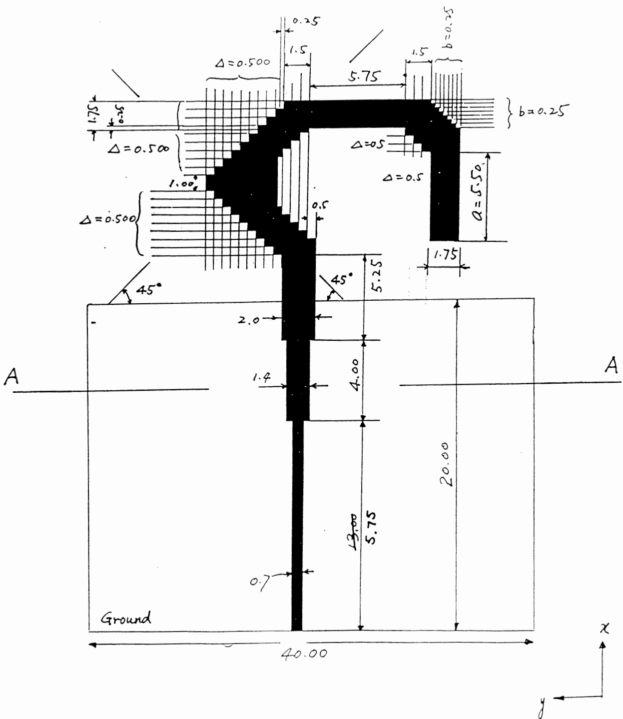
Figure 2. Dimensions of single antenna
