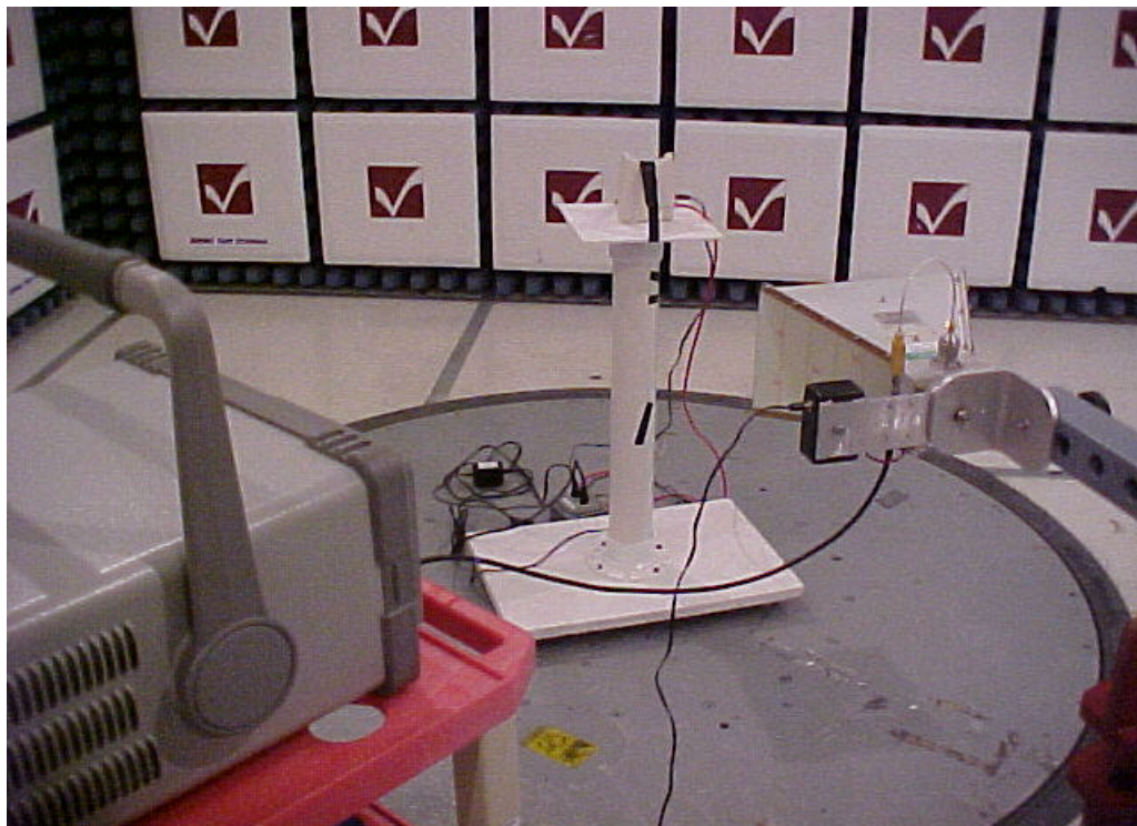
View of the Access Point A1 spread spectrum transceiver during the Radiated Emissions tests.
