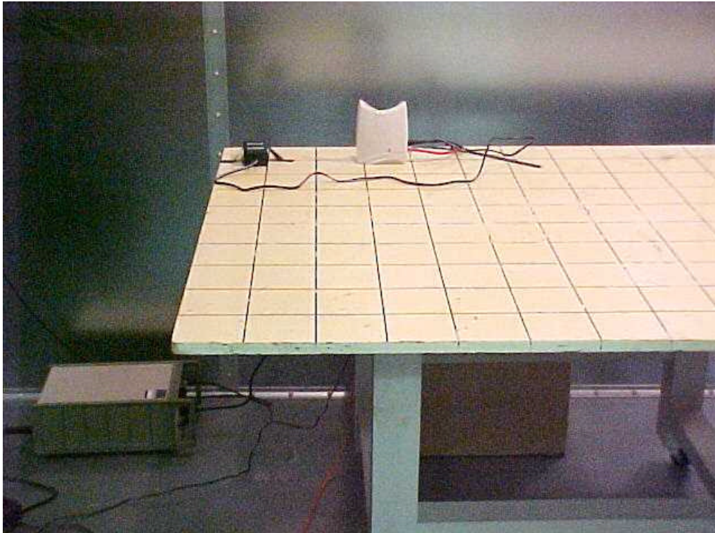
View of the Access Point A1 spread spectrum transceiver during the Conducted Emissions (AC line) tests.
