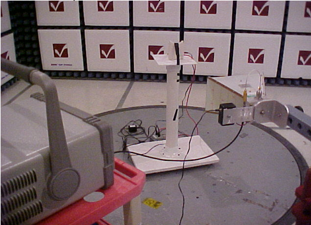
1 meter antenna separation chamber setup
