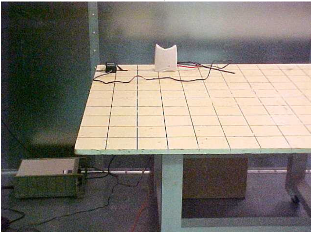
Conducted Emissions in the shielded room, AC line
