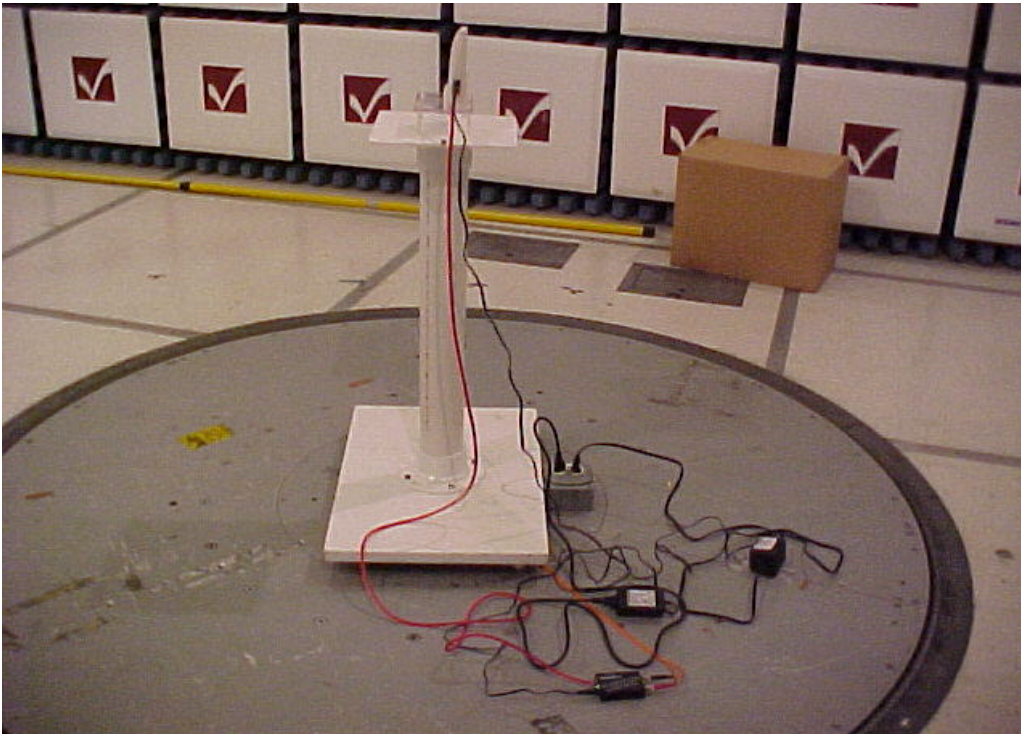
3 meter antenna separation chamber set up
