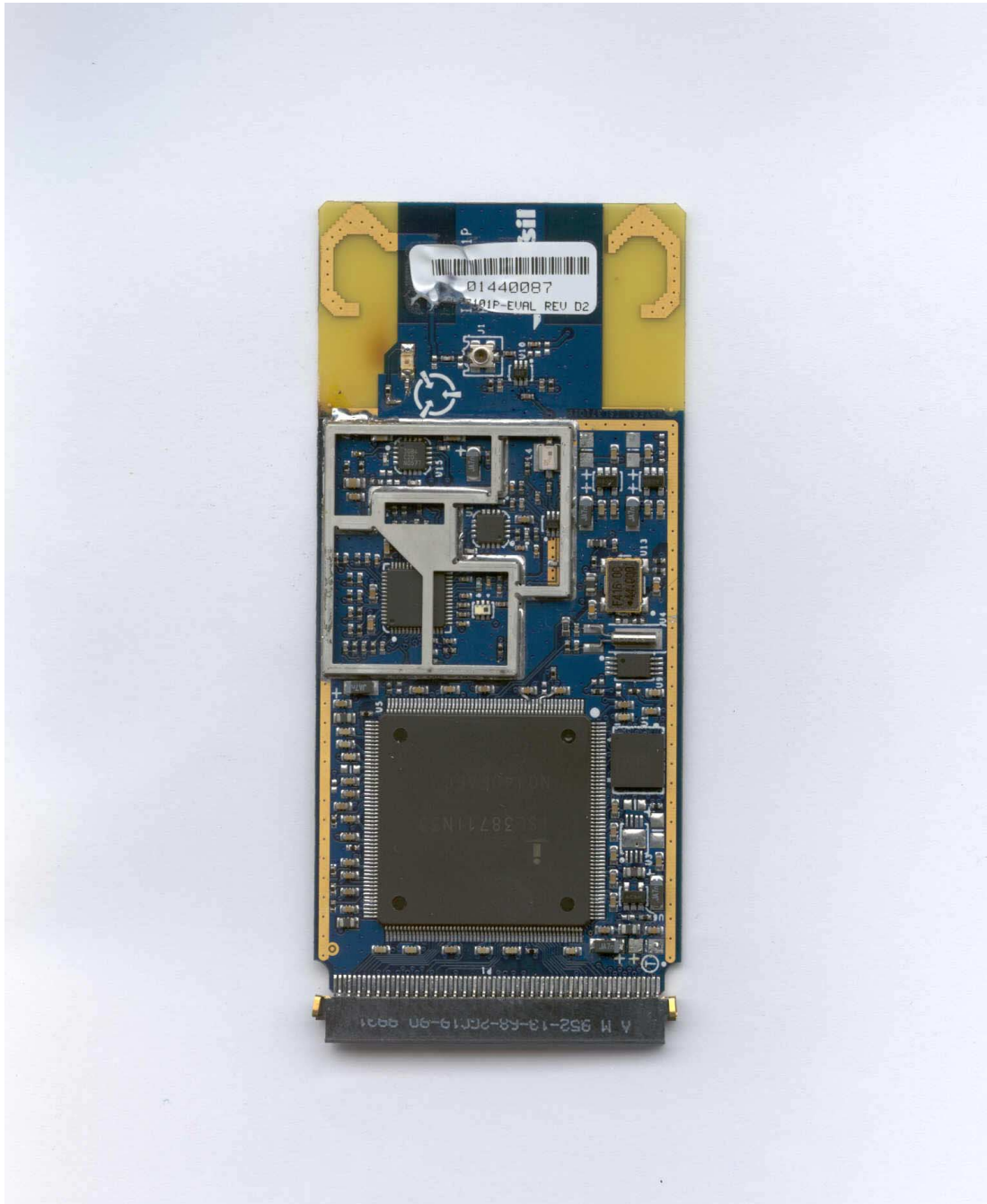
ISL37101P-10 PCB front without shield
