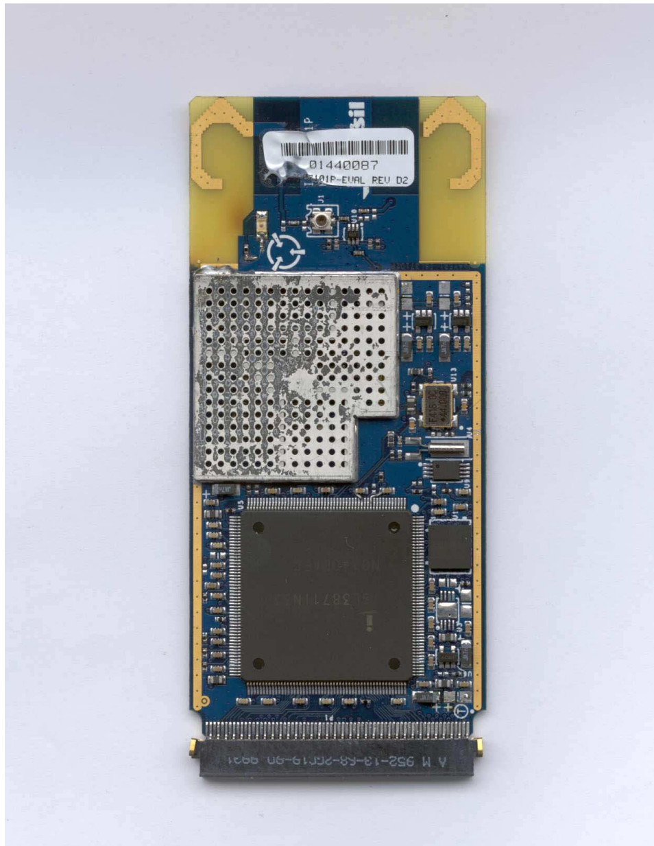
ISL37101P-10 PCB front with shield
