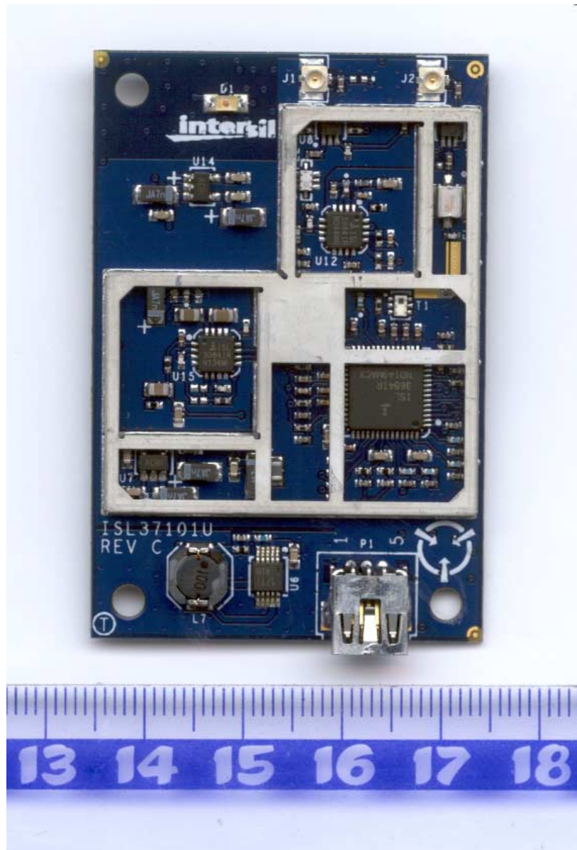
ISL37101U PCB front without shield
