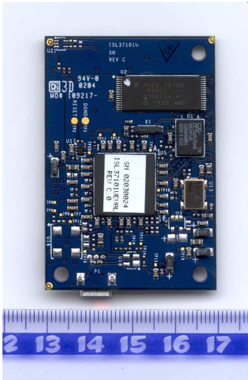
ISL37101U PCB rear
