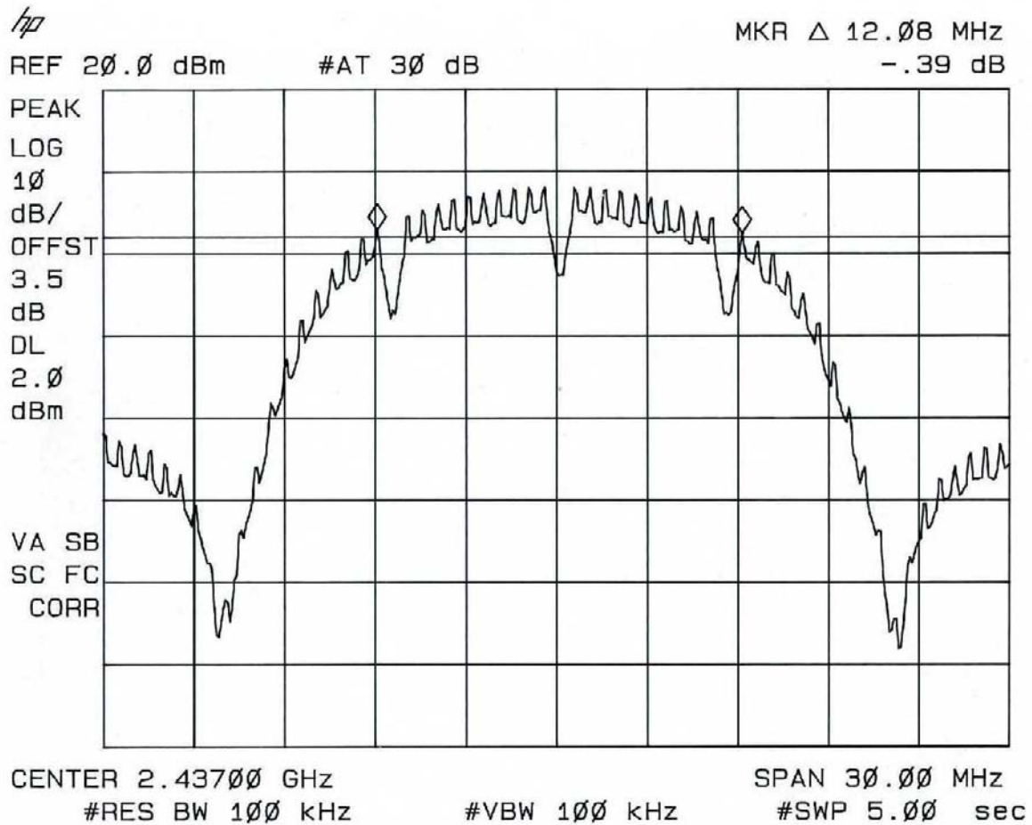
Plot 5 - Minimum 6 dB bandwidth at a transmission bitrate of 1 Mbit/s.
