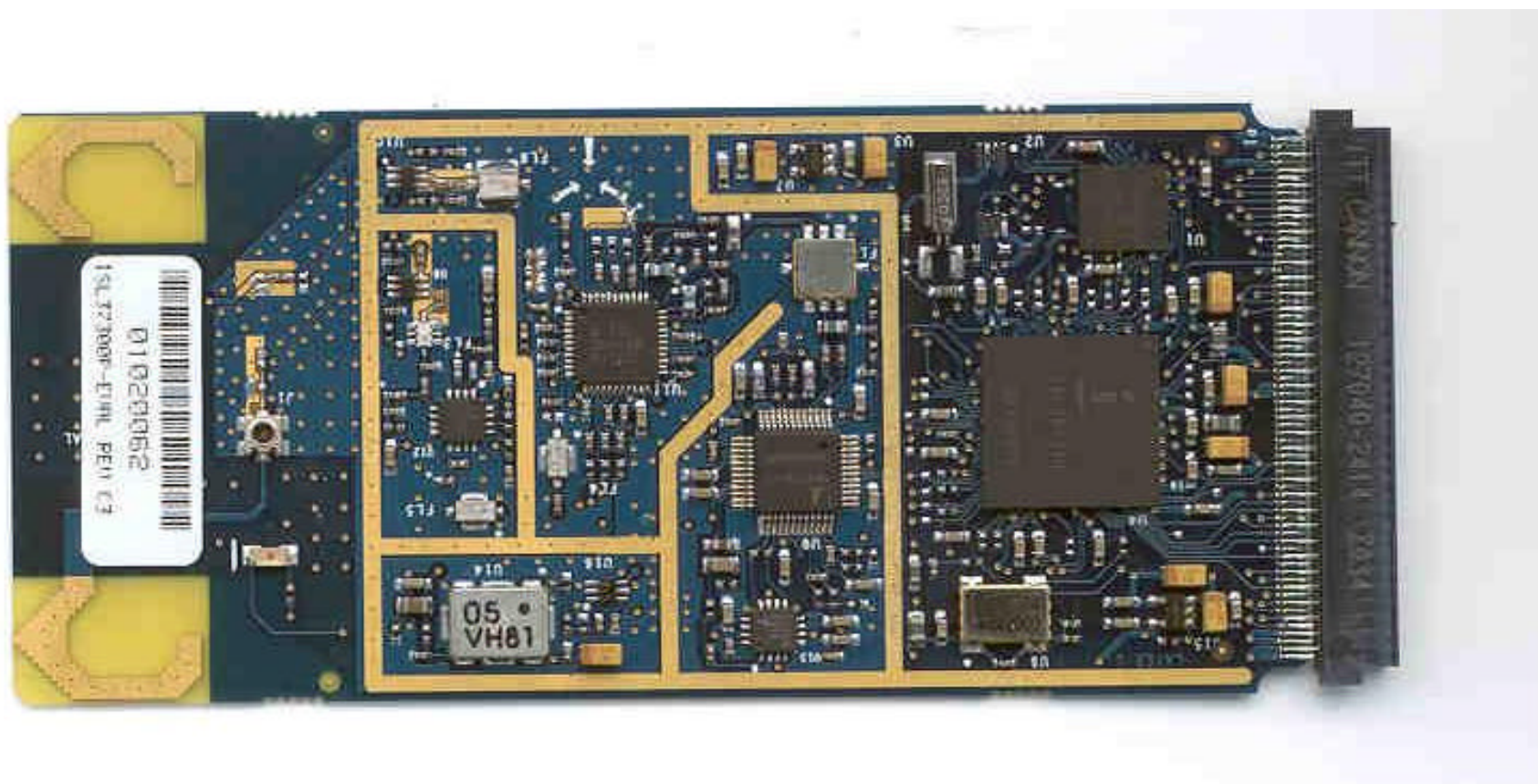
PC BOARD TOP SIDE
