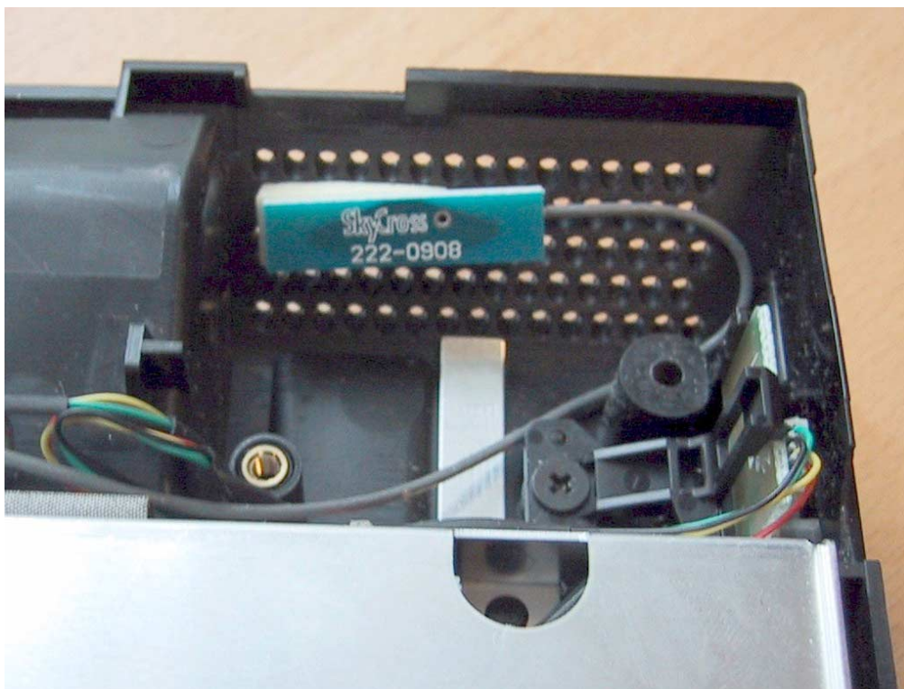
Skycross 5GHz antenna mounted on right lower corner of PC housing
