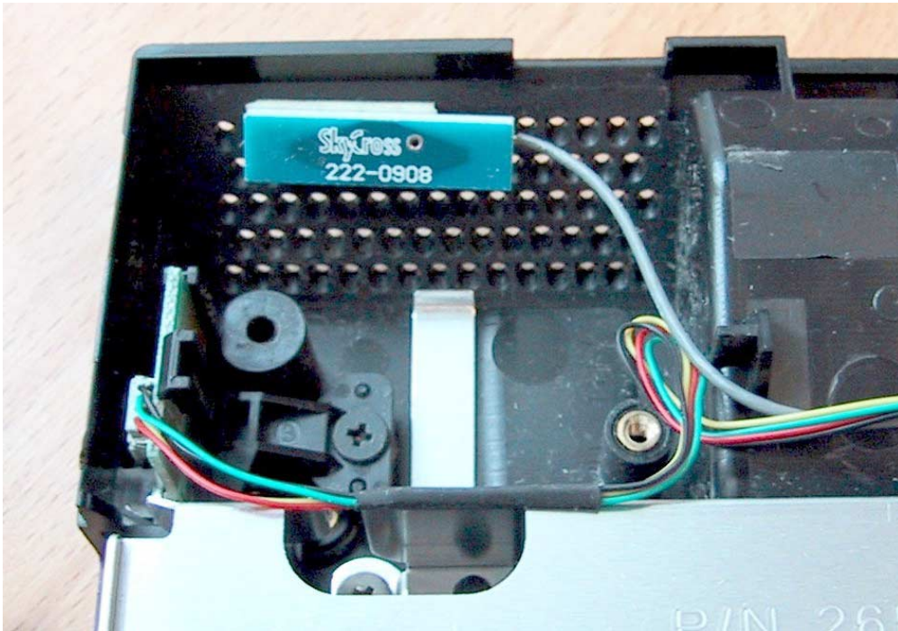
Skycross 5GHz antenna mounted on left lower corner of PC housing
