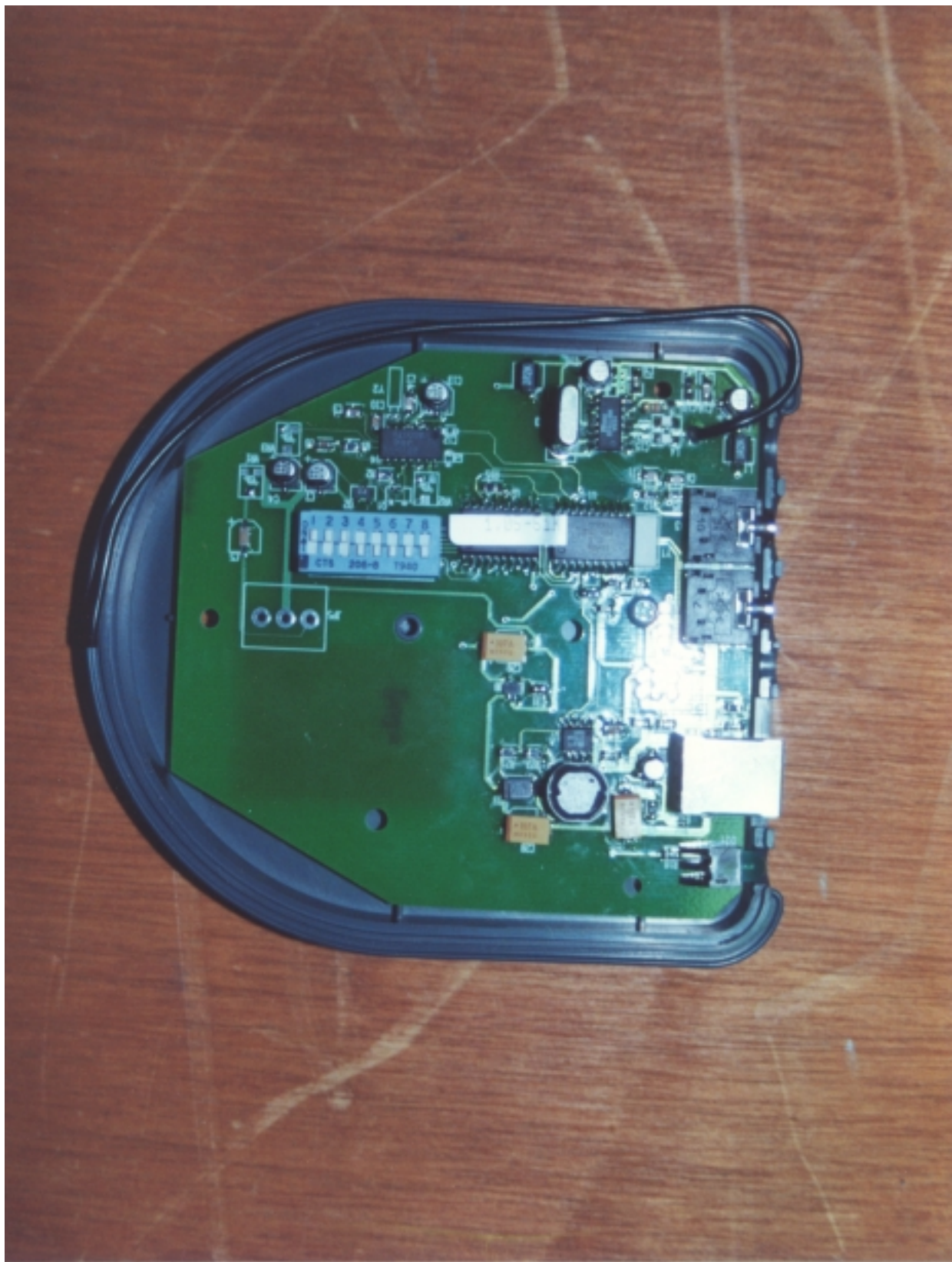
TOP VIEW OF EUT (RECEIVER)
