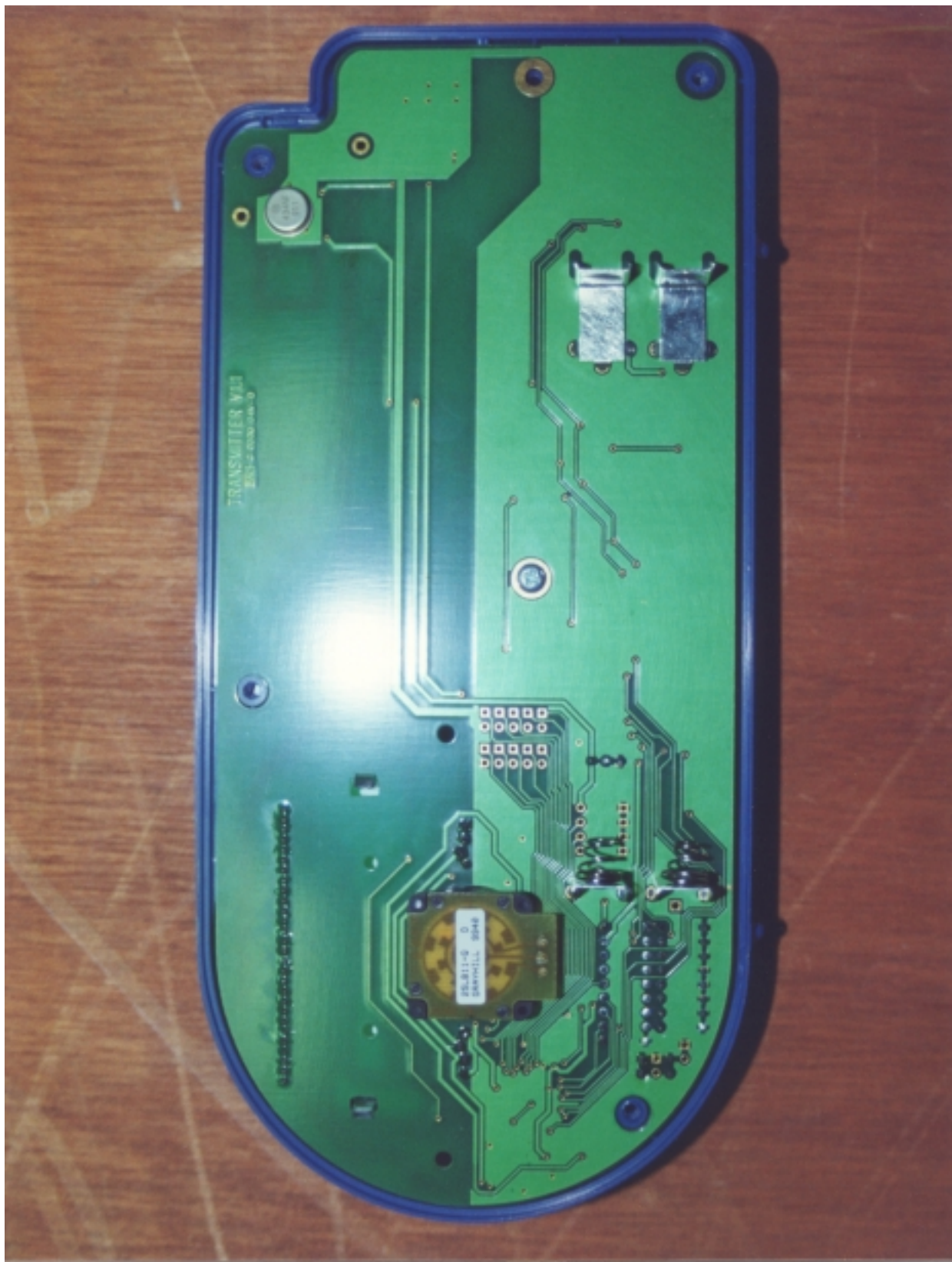
TOP INSIDE VIEW OF EUT (TRANSMITTER)
