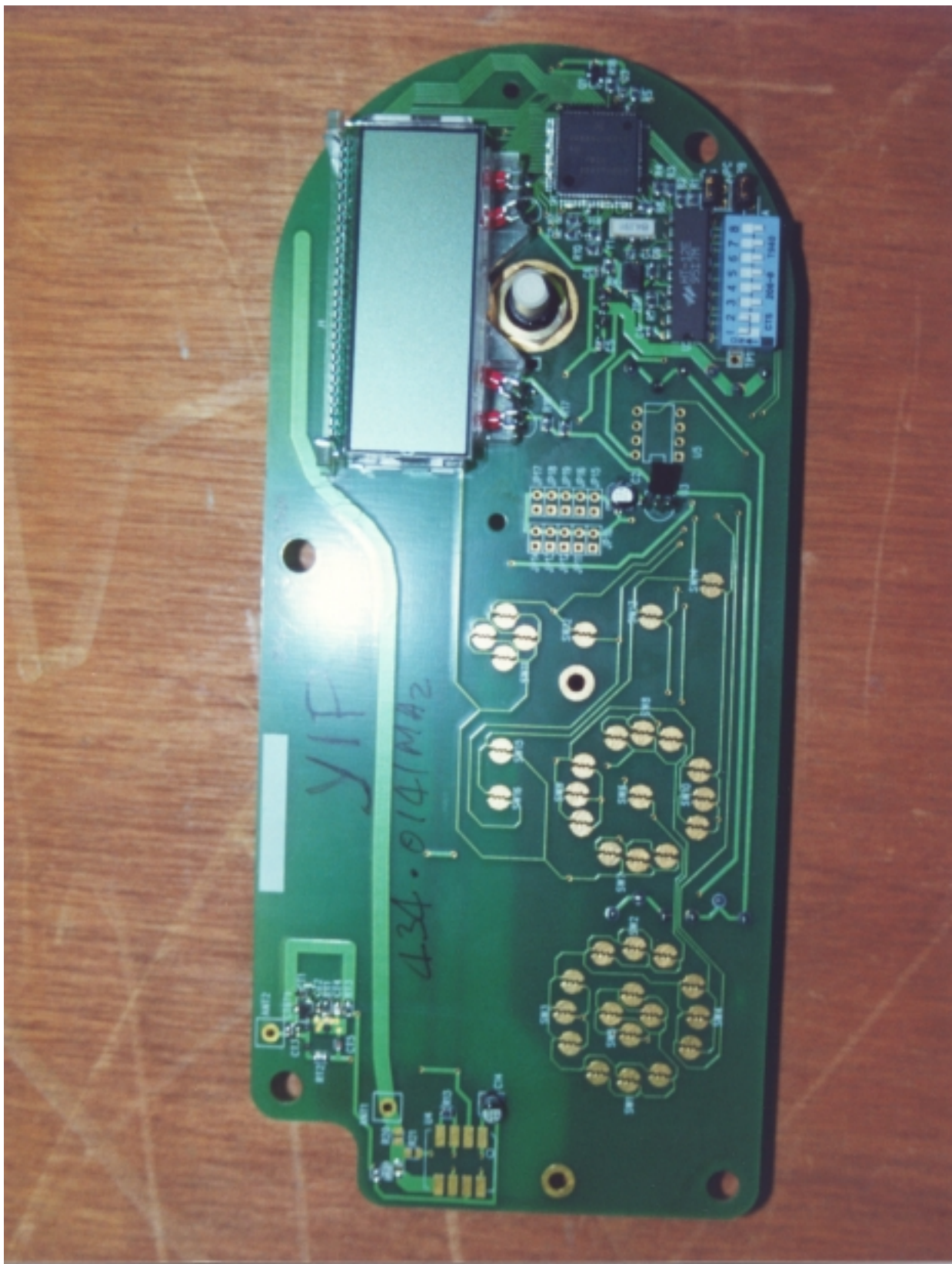
COMPONENT SIDE OF BOARD (TRANSMITTER)
