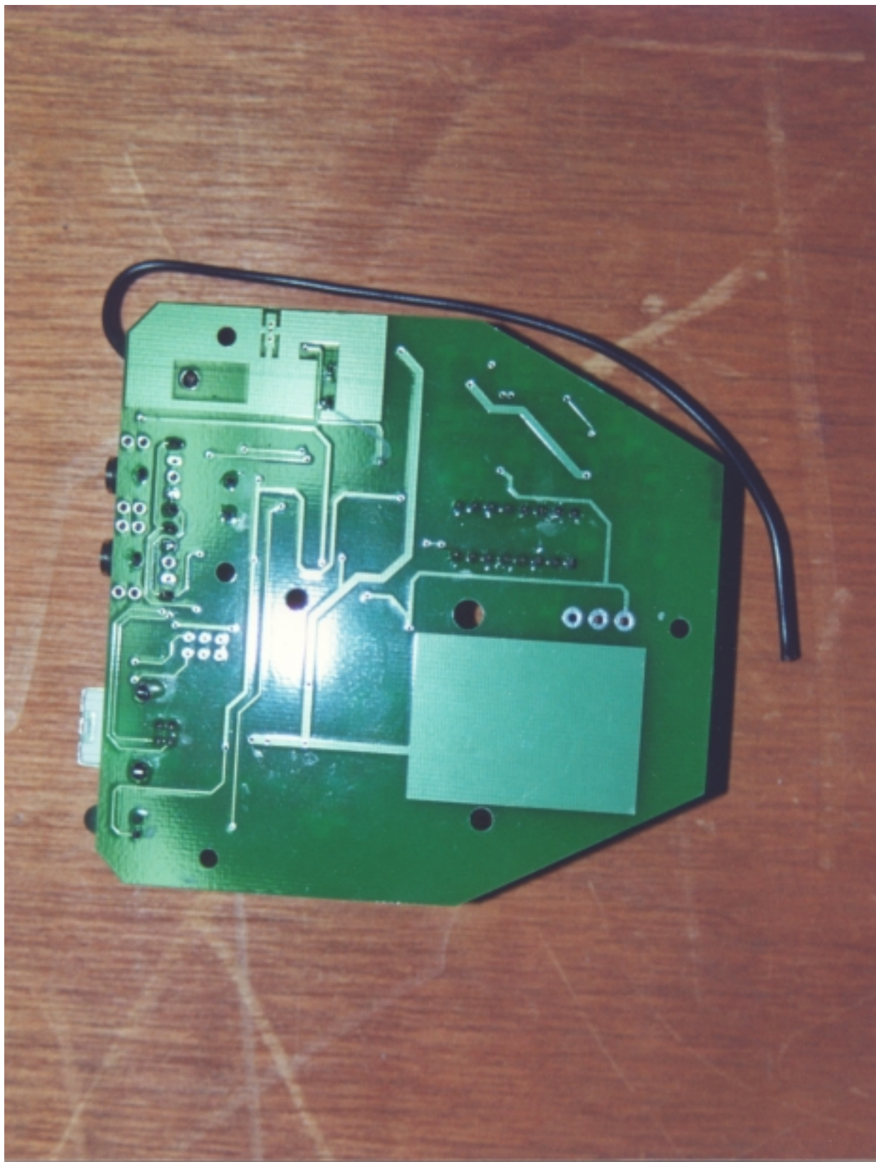
SOLDER SIDE OF BOARD (RECEIVER)
