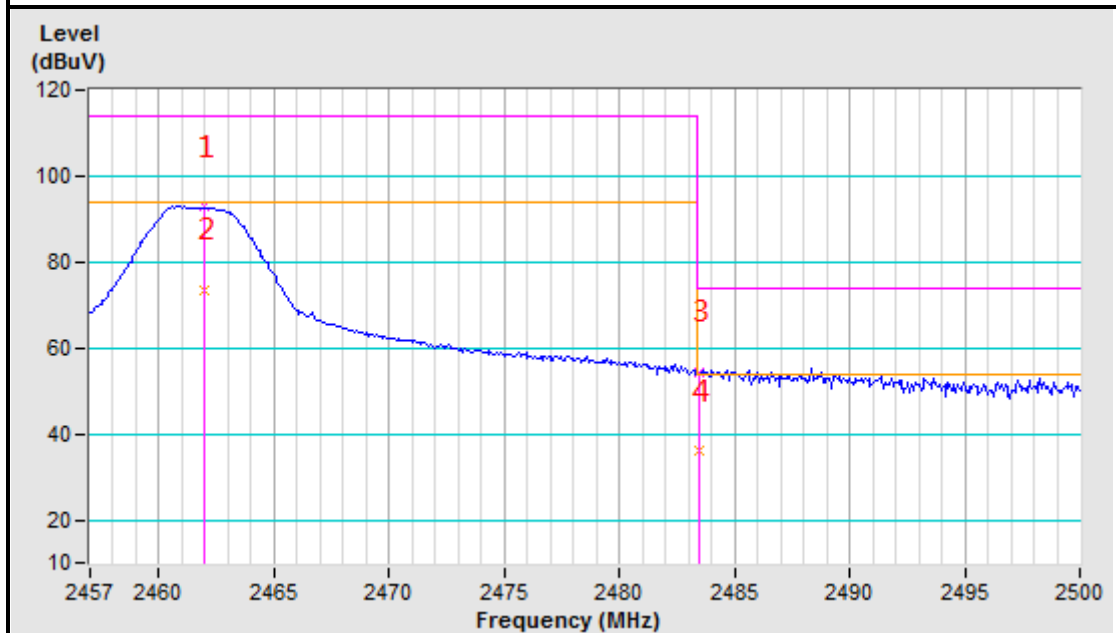
2462MHz Vertical
