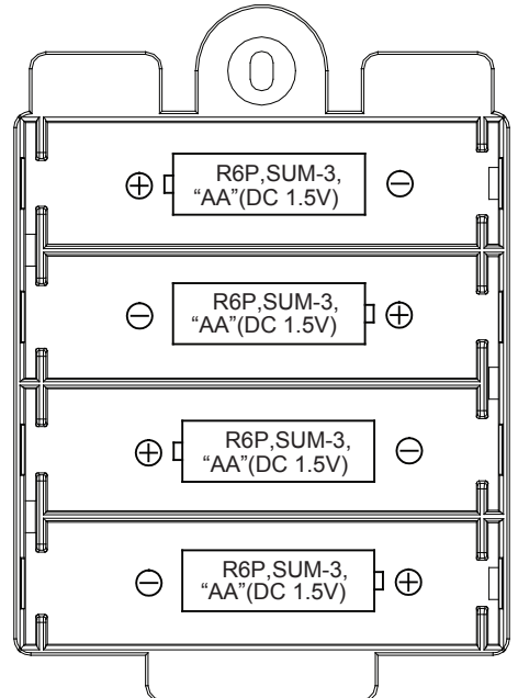
HULK Body Batterybox
