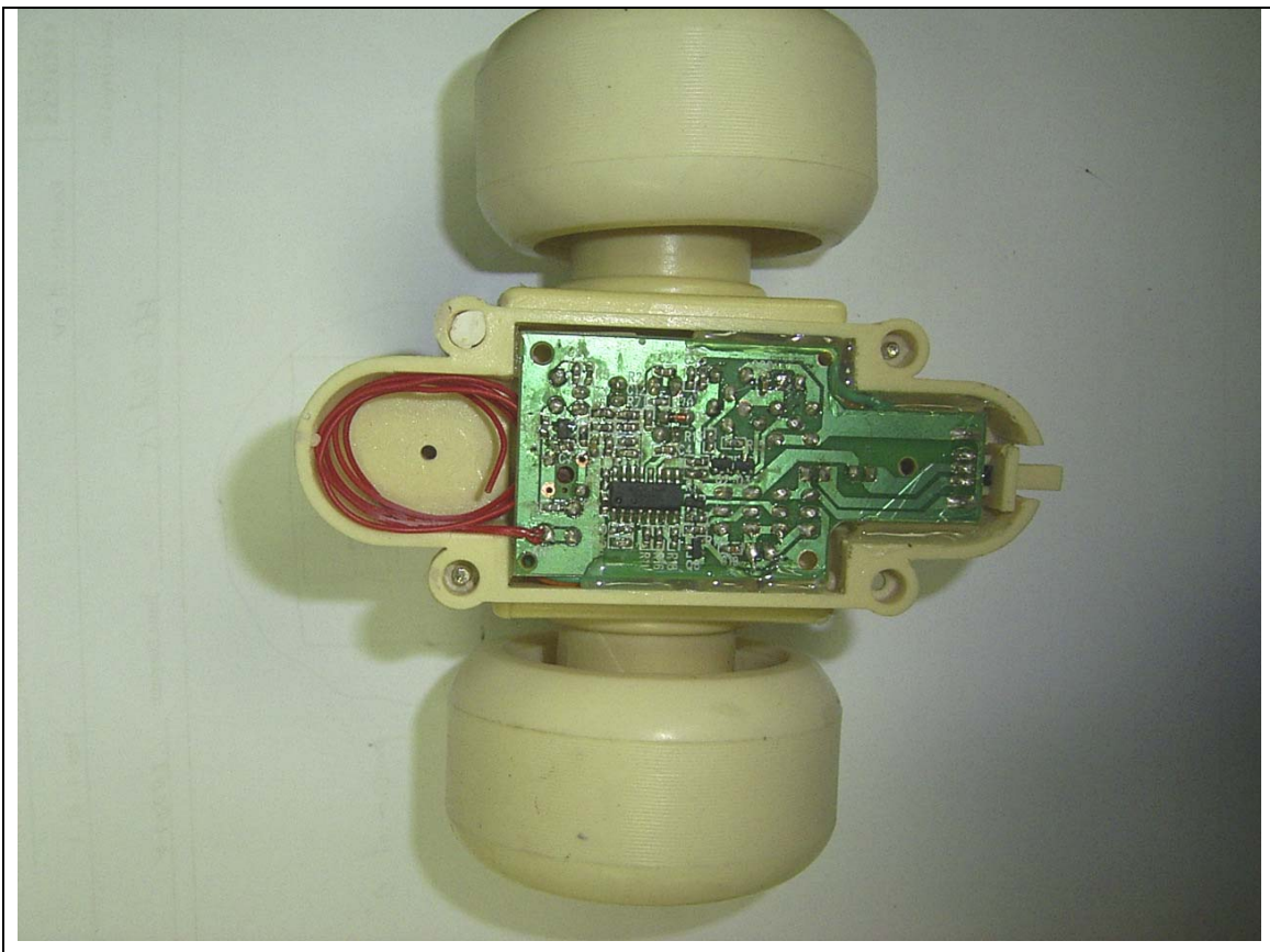
Photo No. 2: The component placement and the assembly
