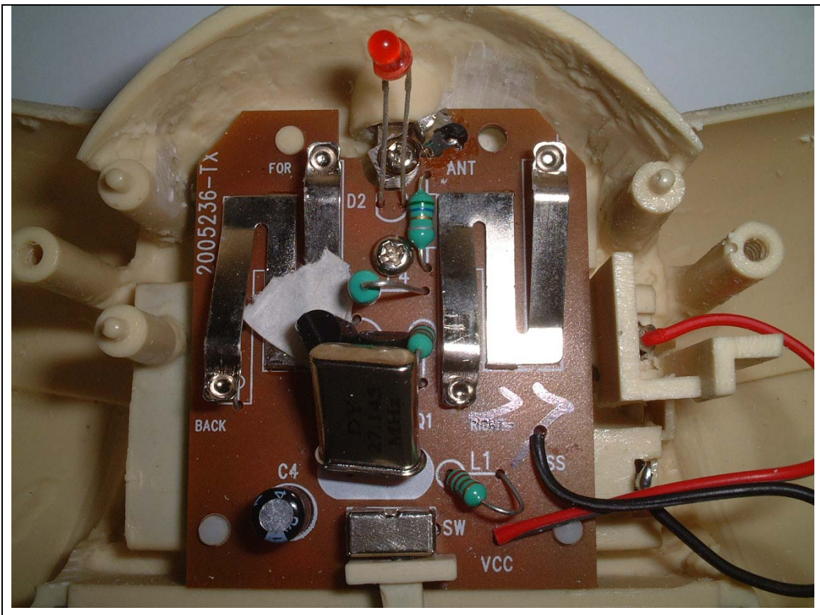
Photo No. 2: PCB Component Side
