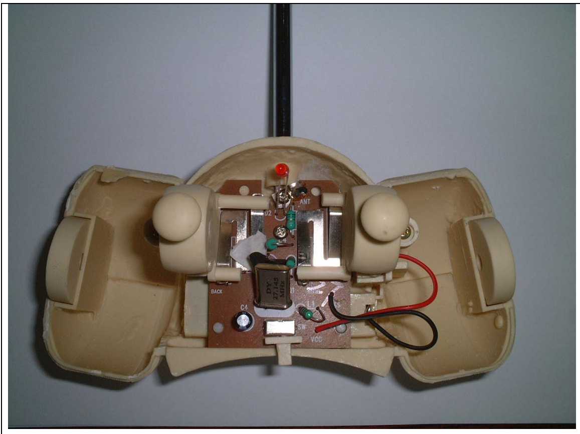
Photo No. 3: The component placement and the assembly
