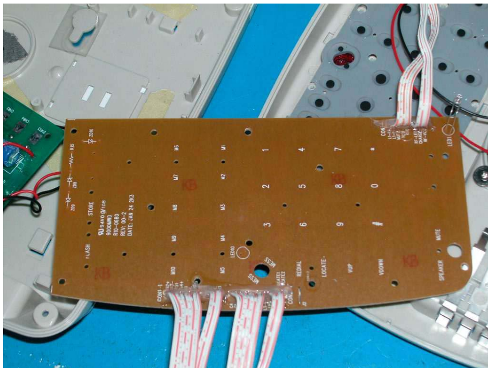
Base keypad rear side
