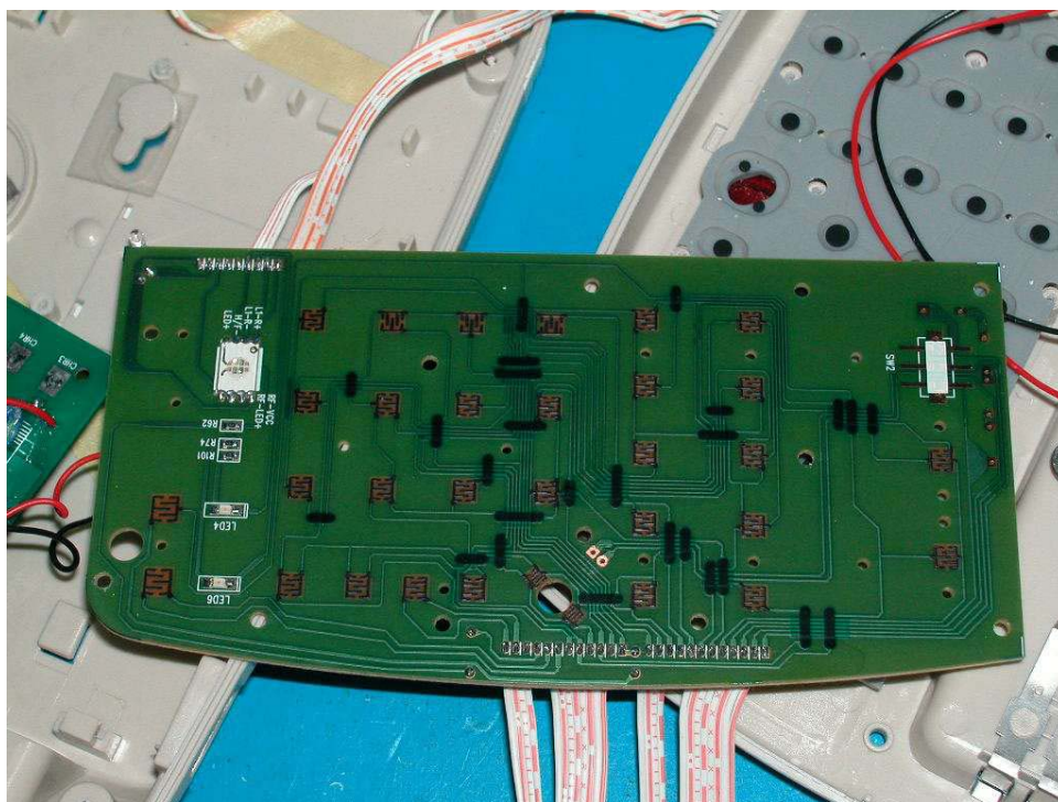
Base keypad front side
